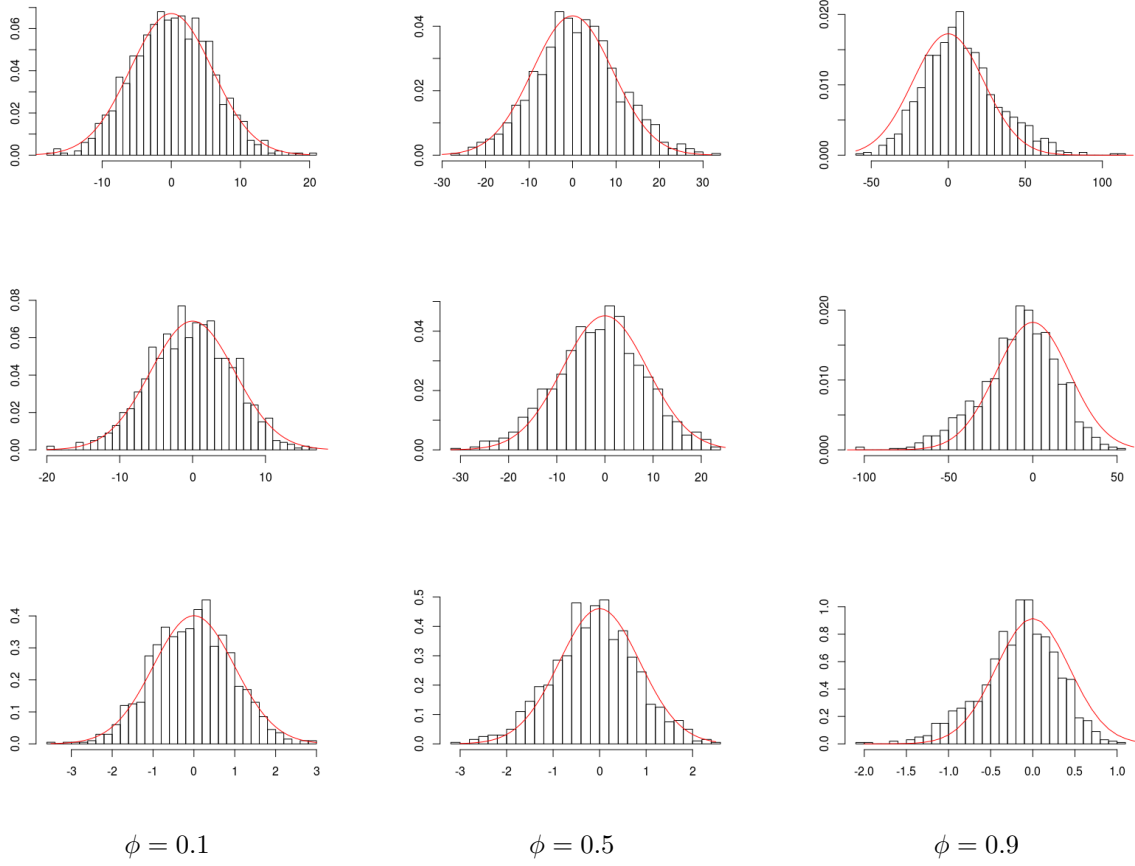
FIGURE 14. Histograms for a = 5 , b = -5 . First row: (\hat{m}_n^{(1)} - m) . Second row: (\hat{b}_n^{(1)} - b) . Third row: (\hat{\phi}_n^{(1)} - \phi) .
