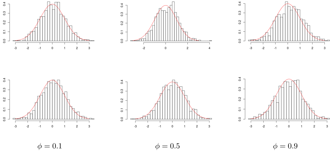
FIGURE 15. Histograms for c = 5 , d = -5 , n = 1000 . First row: (\hat{c}_n^{(1)} - c) . Second row: (\hat{d}_n^{(1)} - d) .
