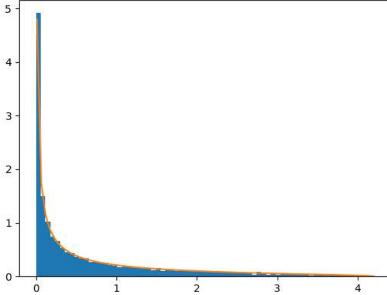
Figure 3: Histogram of the eigenvalues and graph of g_N(x) for M = 500, N = 1500, L = 2
