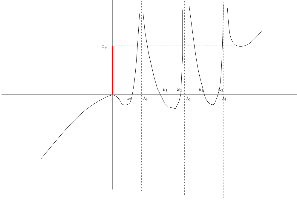
Figure 1: Typical representation of \phi(w) as a function of w for \overline{M} = 3 . There is no local maximum on [\overline{\lambda}_3, \mu_1] and on [\overline{\lambda}_2, \mu_2] , so that \mathcal{S} = [0, x_+] .
