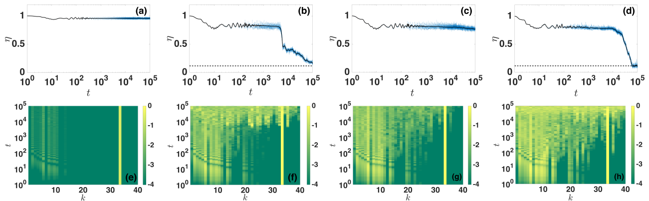
FIG. 10. Same as in Fig. 8 but for the FPUT model. The dashed horizontal line in panels (b) and (d) show the mean value \langle \eta \rangle given by Eq. (12). The values of the energy in this case are H = 0.25 (a)-(e), H = 2.9 (b)-(f), H = 4 (c)-(g), and H = 8.7381 (d)-(h).
