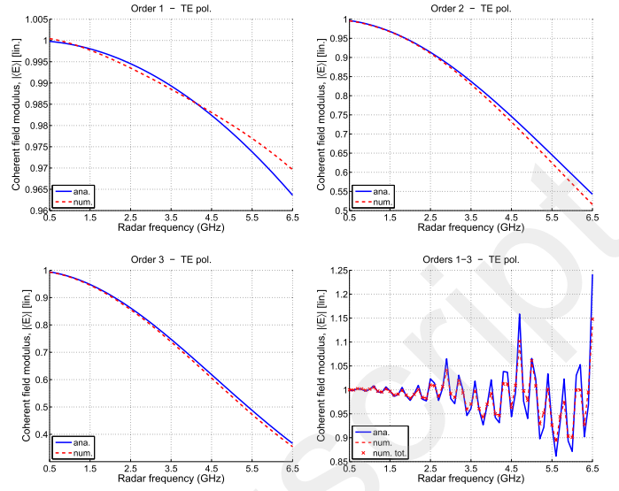
Fig. 6. Modulus of the coherent fields scattered from a multilayered medium of three random rough interfaces under the third configuration, in the frequency band f \in [0.5; 6.5] GHz: comparison of the proposed analytical model with a reference numerical method.
