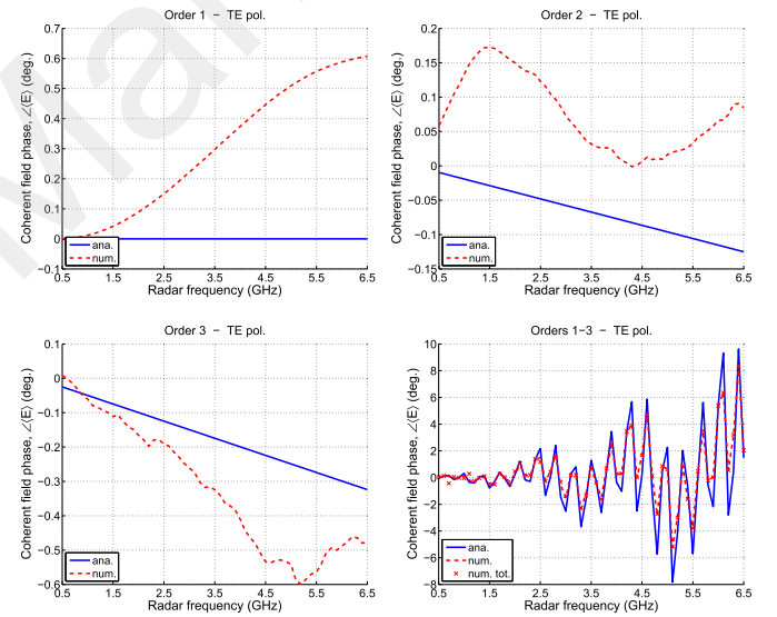
Fig. 7. Phase (in degrees) of the coherent fields scattered from a multilayered medium of three random rough interfaces under the third configuration, in the frequency band f \in [0.5; 6.5] GHz: comparison of the proposed analytical model with a reference numerical method.
