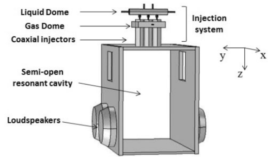
Figure 1. Schematic representation of the experimental set-up: main resonant cavity with two injection domes.
