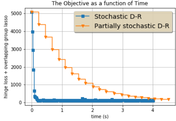
Fig. 1. The objective function F + G as a function of time in seconds for each algorithm
