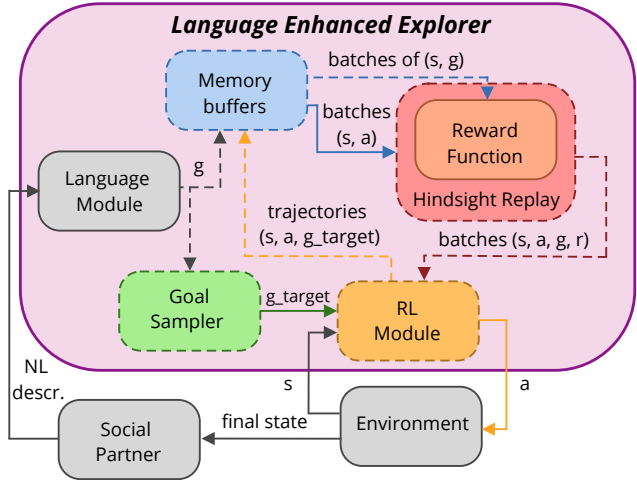
Figure 1: The Language Enhanced Exploration algorithm. Colored dashed circled boxes represent modules that are updated by the LE2 algorithm. Grey boxes represent non-updated modules, some of which are external to the agent (social partner, environment).
