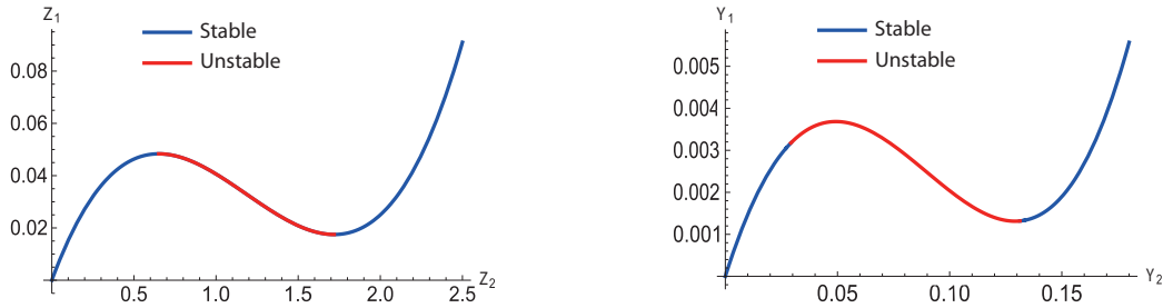
Figure 2: SIM the B-NES (left) and T-NES (right). \kappa_N = 0.6 and \lambda_N = 0.1
