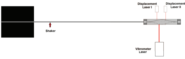
Fig. 13 The scheme of the experimental setup for the measurements with a steel beam as a primary system.
