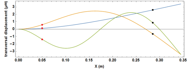
Fig. 15 First three modes of the beam. The red point denotes the point of the forcing application, while the black point shows the point of the absorber attachment.
