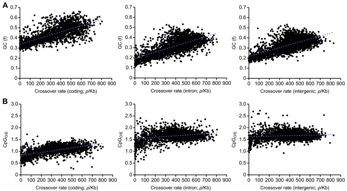
Fig 3. Correlations between recombination rate and GC and CpG content divided according to functional categories. (A) Correlations between recombination rate and GC content in coding (left panel; R^2 = 0.506 , p < 10^{-5} ), intronic regions (centre panel; R^2 = 0.463 , p < 10^{-5} ) and intergenic regions (right panel; R^2 = 0.446 , p < 10^{-5} ). (B) Correlations between recombination rate and CpG O/E in coding (left panel; R^2 = 0.369 , p < 10^{-5} ), intronic regions (centre panel; R^2 = 0.066 , p < 10^{-5} ) and intergenic regions (right panel; R^2 = 0.011 , p = 0.00037 ). 100 kb genomic windows are used in each comparison.
