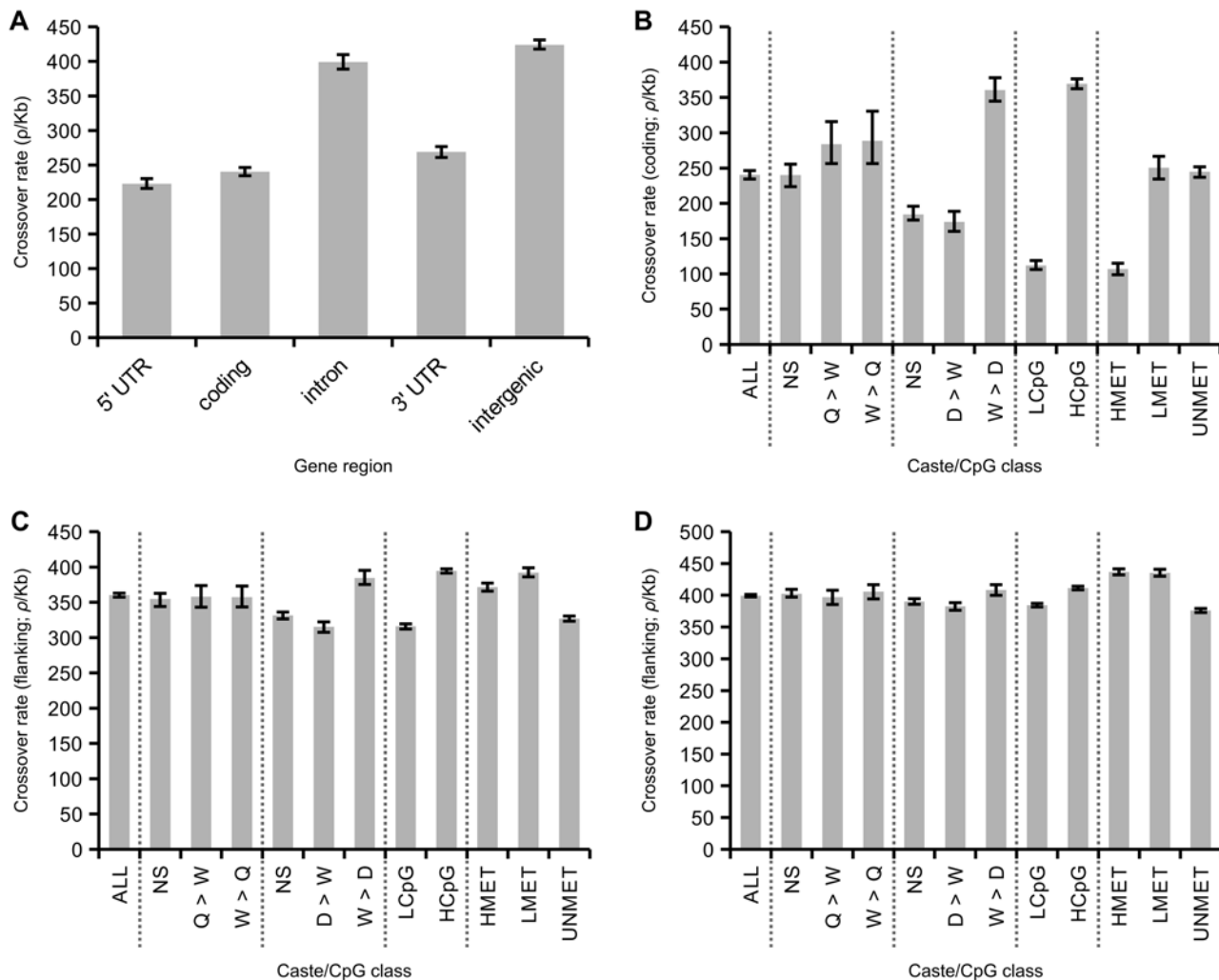
Fig 4. Associations between caste biased gene expression and inferred methylation patterns in honeybees. (A) Variation in average recombination among gene regions. Recombination is significantly reduced in 5' and 3' UTRs and coding regions compared with intronic and intergenic regions. (B) Average recombination rate in coding sequence of all genes (left; ~13,000 genes) and from genes divided according to gene expression patterns and CpG content. Two expression datasets are used. One identifies elevated expression in queens compared to workers (Q>W), workers compared to queens (W>Q) or not significantly different between these two castes (NS). The other that identifies elevated expression in drones compared to workers (D>W), workers compared to drones (W>D) or not significantly different between these two castes (NS). Genes are categorised as either low CpG O/E (LCpG) or high CpG O/E (HCpG) in their coding sequence. Genes are also divided according to experimentally measured levels of germline methylation: highly methylated (HMET), lowly methylated (LMET) and unmethylated (UNMET). (C) Recombination rates in noncoding regions flanking genes. Rates are inferred from noncoding regions of 50 kb starting at 10 kb away from either side of a gene to reduce the influence asserted by genic recombination properties. 95% confidence intervals generated from 200 bootstrap subsamples of all genes attributed to a particular gene class. (D) The same as C but using windows of 100 kb starting at 50 kb from each gene.
