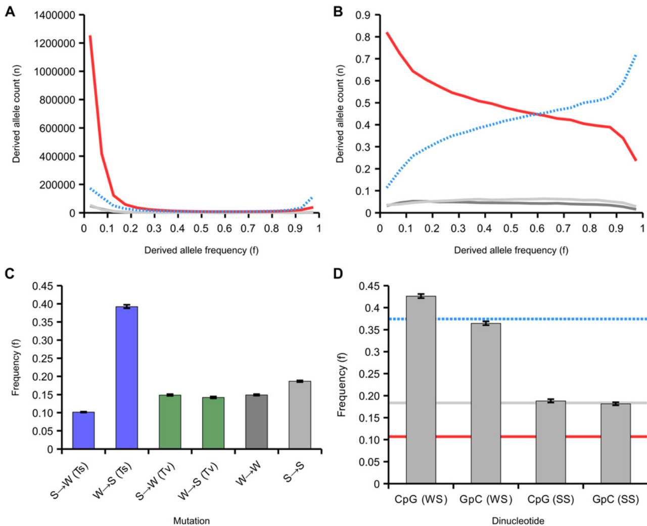
Fig 5. Site frequency spectrum of derived variants. (A) The site frequency spectra of 2,983,700 variants classified according to their mutational origin as defined by comparison to the outgroup. Variants are: SW (strong-to-weak; red line; 2,037,148 SNPs in total); WS (weak-to-strong; blue dashed line; 719,365 SNPs); SS (strong-to-strong; light grey; 117,806 SNPs); WW (weak-to-weak; dark grey; 109,381 SNPs). (B) The relative site frequency spectra of the four variants (variants and colours as in A). (C) Average frequencies of derived variants of different mutational classes. SW and WS mutations are classified as transitions (Ti, blue) or transversions (Tv, green), SS and WW as in A. (D) Average frequency of WS and SS variants that create CpG sites compared to those that create GpC sites. The blue dashed line represents the mean frequency of WS variants, the red line is the mean frequency of SW variants and the grey line is the mean frequency of SS variants. 95% confidence intervals generated from 200 bootstrap subsamples of all SNPs attributed to a particular class.
