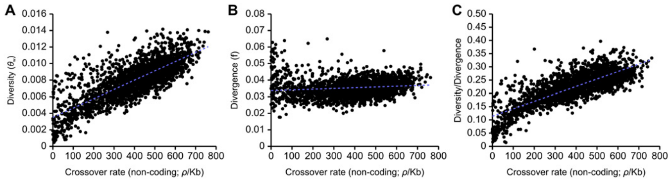
Fig 2. Correlations between estimates of non-coding genetic diversity and divergence with population recombination rates inferred with LDHAT. (A) Correlation between recombination and diversity ( R^2 = 0.615 , p < 10^{-5} ). Linear regression: f(x) = (1.118 \times 10^{-5})x + (3.517 \times 10^{-3}) . (B) Correlation between recombination and divergence between A. mellifera and A. cerana ( R^2 = 0.0185 , p < 10^{-5} ). Linear regression: f(x) = (4.439 \times 10^{-6})x + (3.360 \times 10^{-2}) . (C) Correlation between recombination and diversity/divergence ( R^2 = 0.617 , p < 10^{-5} ). Linear regression: f(x) = (2.801 \times 10^{-4})x + (1.140 \times 10^{-1}) . 100 kb genomic windows are used in each comparison.
