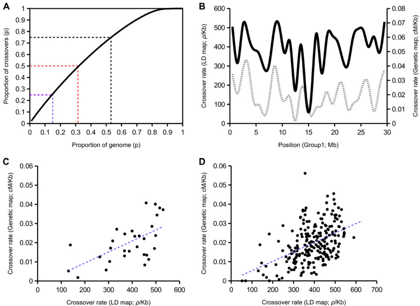
Fig 1. Population recombination rates inferred from linkage disequilibrium among SNPs using LDHAT in comparison with a genetic map [3]. (A) Proportion of recombination as a function of the proportion of genome in which it occurs. (B) Variation in recombination rates along the large metacentric chromosome Group1 (LD map: solid black line; genetic map from [3]: grey dashed line). The maps are transformed to the same resolution of 1 Mb windows. (C) Correlation between recombination rates in the LD-based map and genetic map from [3] ( R^2 = 0.341 ; p = 0.000424 ) across chromosome Group1 in windows of 1 Mb. (D) Correspondence between the two maps across the whole genome in windows of 1 Mb ( R^2 = 0.213 ; p < 10^{-5} ).
