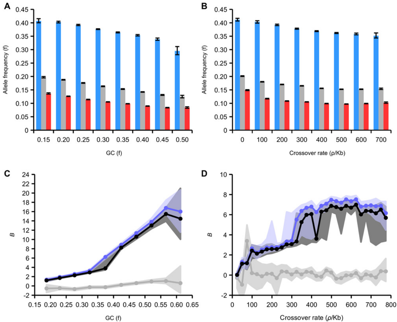
Fig 6. Effect of GC content and recombination on derived allele frequencies in intergenic regions. (A) Average allele frequency of all, WS, SW variants relative to GC content. 95% confidence intervals generated from 200 bootstrap subsamples of all SNPs attributed to a particular GC bin. (B) Average allele frequency of all, WS, SW variants relative to recombination. 95% confidence intervals generated from 200 bootstrap subsamples of all SNPs attributed to a particular rate bin. (C) Maximum likelihood estimation of B , the gBGC coefficient, derived from the site frequency spectrum plotted against GC content (black line, all variants; blue line, transitions; grey line, transversions). (D) Maximum likelihood estimates of B relative to recombination rate (variants and colours as in C).
