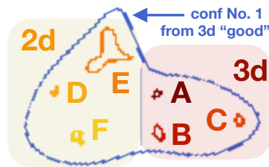
FIG. 3. The examples A, B, \dots , F of the deformed circles for which the neural network makes the worst predictions (given in Table III). For comparison, we plot – keeping the correct scale – the configuration No. 1 from the good examples for the 3d model shown in the upper plot of Fig. 2.
