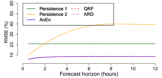
Fig. 8. RMSE of the models depending on the horizon
