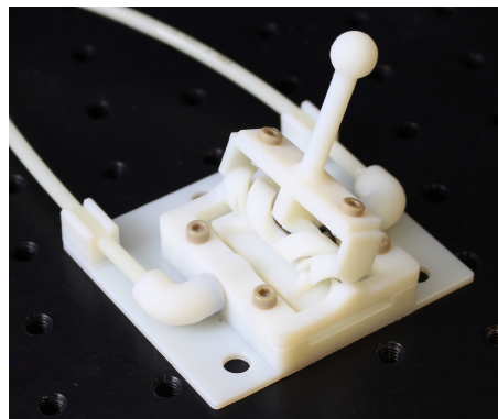
Fig. 13: Prototype of 3D-printed hydraulic revolute joint.
