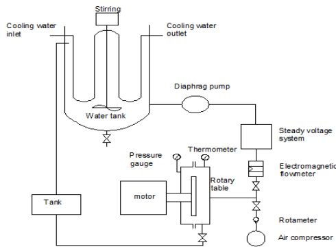
Figure 1. Rotary spray erosion testbed
