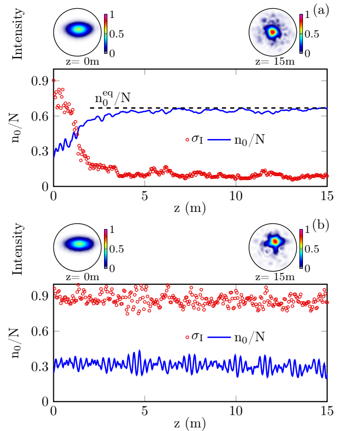
FIG. 3: Disorder-induced beam cleaning: Numerical simulations of the NLS Eq.(8) showing the evolutions of the relative variance of intensity fluctuations \sigma_I(z) from Eq.(33) (red circles), and condensate fraction n_0(z)/N (blue line), in the presence of disorder (a), and in the absence of disorder (b). The intensity patterns I(\mathbf{r}) inside the fiber core (circles) are shown at z = 0 and z = 15\text{m} . The horizontal dashed black line in (a) shows the condensate fraction at thermal equilibrium, n_0^{\text{eq}}/N \simeq 0.68 (from Eq.(31)). The disorder induces a stable beam cleaning condensation characterized by a significant reduction of intensity fluctuations down to \sigma_I \simeq 0.1 (a), which is in contrast with the case without disorder where the variance of intensity fluctuations remain almost constant throughout propagation with \sigma_I \simeq 0.9 . Parameters are: \Delta\beta = 2.6\text{m} ( 2\pi/\sigma_\beta = 2.13\text{m} , l_\beta = 30\text{cm} ), N_* = 120 modes, a = 26\mu\text{m} , N = 47.5\text{kW} .
