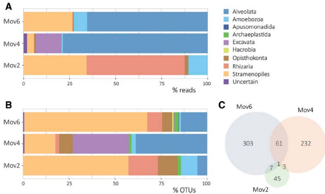
Fig. 2. Relative abundance of microbial eukaryotes in Movile Cave samples. A. Relative abundance of 18S rRNA gene amplicon reads. B. Relative abundance of operational taxonomic units (OTUs). C. Venn diagrams showing specific and shared OTUs among samples.
