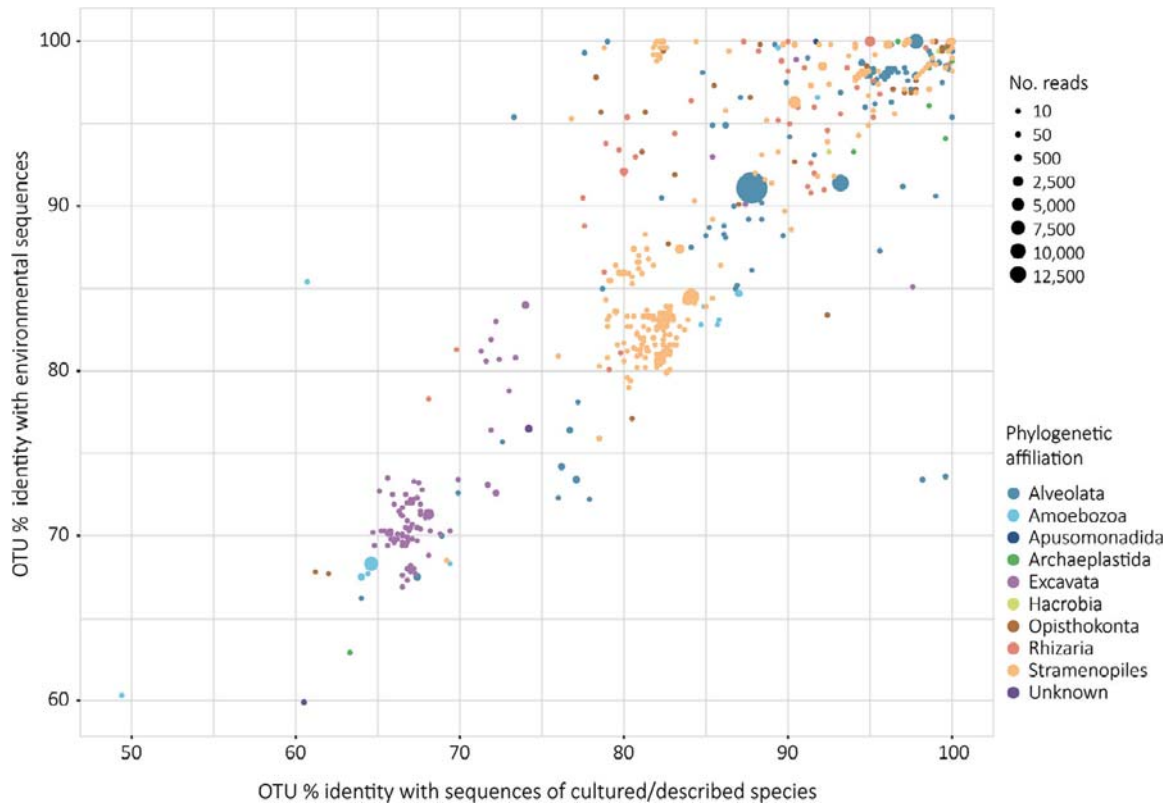
Fig. 3. Divergence plots of eukaryotic OTUs from the Movile Cave with respect to 18S rRNA gene sequences of cultured/described protists and environmental surveys. The size of the dots is proportional to the number of reads. Their colour indicates their phylogenetic affiliation.
