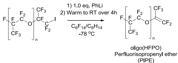
Scheme 1: The formation of PIPE using oligo(hexafluoropropylene oxide) primary iodide and phenyl lithium in a 50/50 mole ratio of hexane and perfluorohexane.
