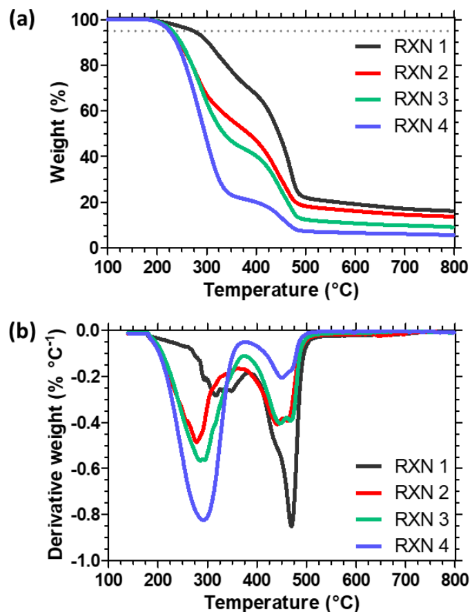
Figure 2: Thermal gravimetric analysis thermograms, under nitrogen, of poly[VDF- g -oligo(HFPO-PIPE)] graft copolymers: weight loss (a) and first derivative of the weight (b) as a function of temperature.
