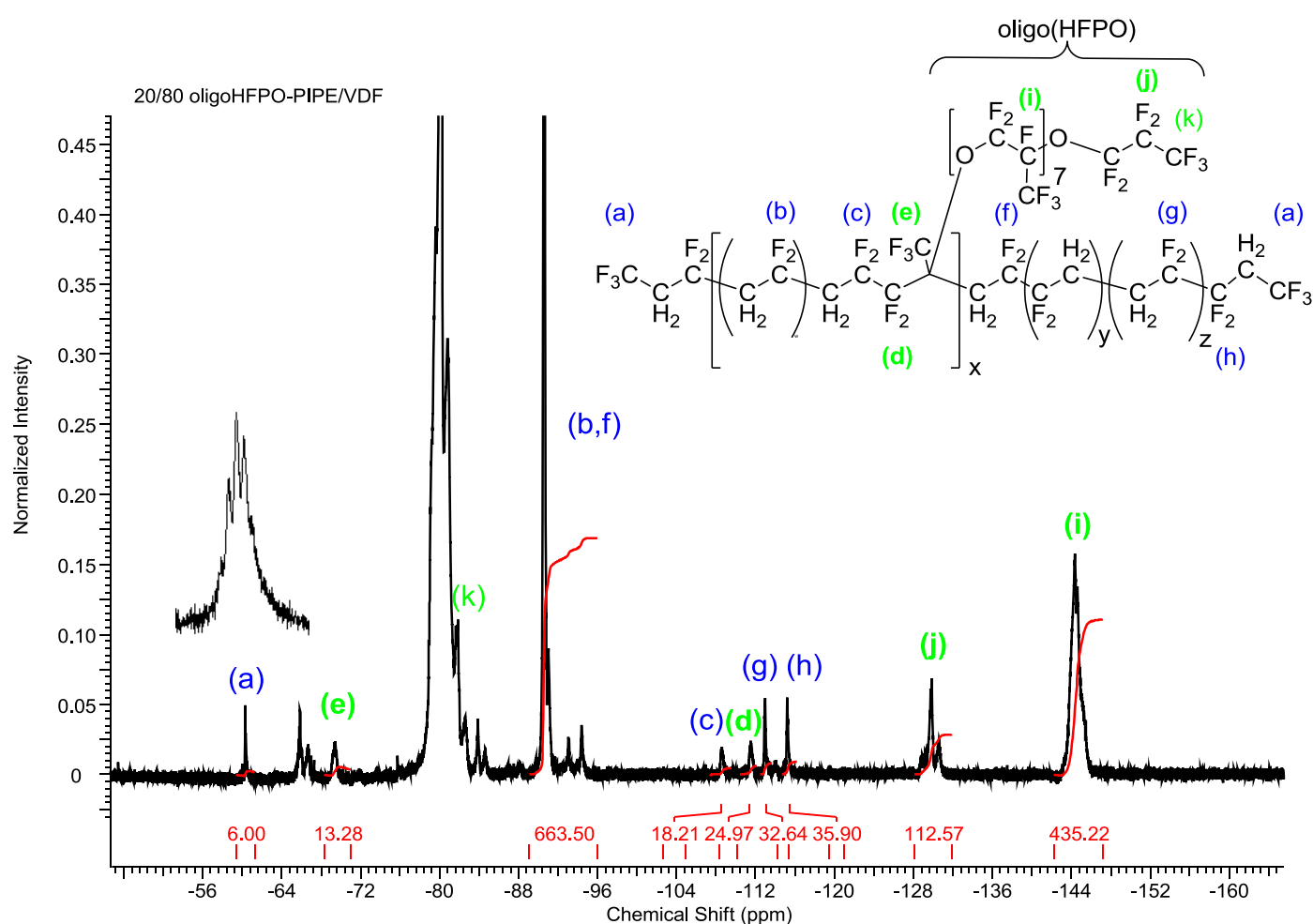
Figure 1. 19 F-NMR spectrum of Poly[VDF-g-oligo(HFPO)] graft copolymer (RXN #4, Table 1) using acetone as the solvent and a C 6 D 6 capillary.
