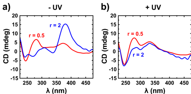
Figure 4. Circular dichroism spectra of AzoDiGua in the presence of ct-DNA (50 \mu M in 10 mM phosphate buffer, pH = 7.0) at AzoDiGua:DNA ratio r = 0.5 (red) and r = 2.0 (blue), before (a, -UV) and after (b, +UV) irradiation at 365 nm for 8 min. T = 22 °C.
