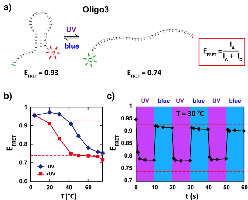
Figure 6. Reversible photocontrol of DNA nanostructure assembly at constant temperature. (a) Oligo3 is a self-complementary hairpin oligonucleotide labeled with a donor D (fluorescein) and an acceptor A (Texas Red) of Förster resonance energy transfer (FRET). The FRET efficiency ( E_{\text{FRET}} ), calculated from the fluorescence intensities of the acceptor ( I_A ) and of the donor ( I_D ), decreases/increases upon melting/hybridization of the self-complementary sequences. (b) Oligo3 melting followed by E_{\text{FRET}} measurement as a function of temperature, with (+UV) or without (-UV) illumination at 365 nm. The dashed lines indicate the E_{\text{FRET}} values at which Oligo3 is hybridized ( E_{\text{FRET}} = 0.93 ) and melted ( E_{\text{FRET}} = 0.74 ) in the absence of AzoDiGua. (c) E_{\text{FRET}} of Oligo3 in the presence of AzoDiGua, as a function of time, for successive cycles of UV (365 nm) and blue (440 nm) illumination performed at a constant temperature T = 30 °C. [Oligo3] = 33 \mu\text{M} in 10 mM Tris buffer pH 7.4 + 50 mM NaCl; [AzoDiGua]:Oligo3 ratio r = 1 .
