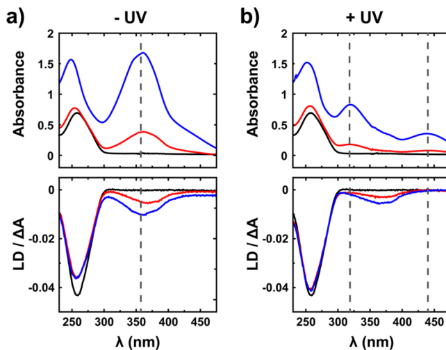
Figure 5. Absorption (top) and linear dichroism (bottom) spectra of AzoDiGua in the presence of ct-DNA (50 \mu M in 10 mM phosphate buffer, pH = 7.0) at AzoDiGua:DNA ratio r = 0 (black), r = 0.5 (red), and r = 2.0 (blue), before (a, -UV) and after (b, +UV) irradiation at 365 nm for 8 min. The dashed lines indicate the maxima of absorption of trans -AzoDiGua (a, 357 nm) and cis -AzoDiGua (b, 319 and 440 nm).
