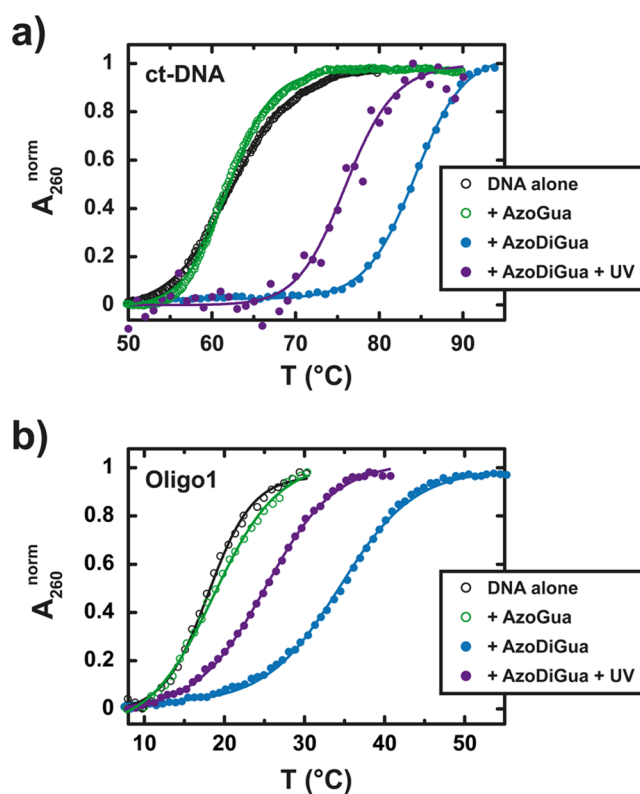
Figure 3. AzoDiGua affects the melting of DNA in a photodependent manner. Thermal denaturation profiles of (a) ct-DNA ( 40.0 \mu\text{M} in 10 mM Tris buffer, pH = 7.4) and (b) Oligo1 ( 20.0 \mu\text{M} in 10 mM Tris buffer + 5 mM NaCl, pH = 7.4) in the presence of AzoGua and AzoDiGua without or with illumination at 365 nm (+UV) during the acquisition of the melting curve (a) or for 1 min before the measurement (b). The PGD concentrations are 20 \mu\text{M} (a) and 40 \mu\text{M} (b). Solid lines represent sigmoidal fits of the experimental data.
