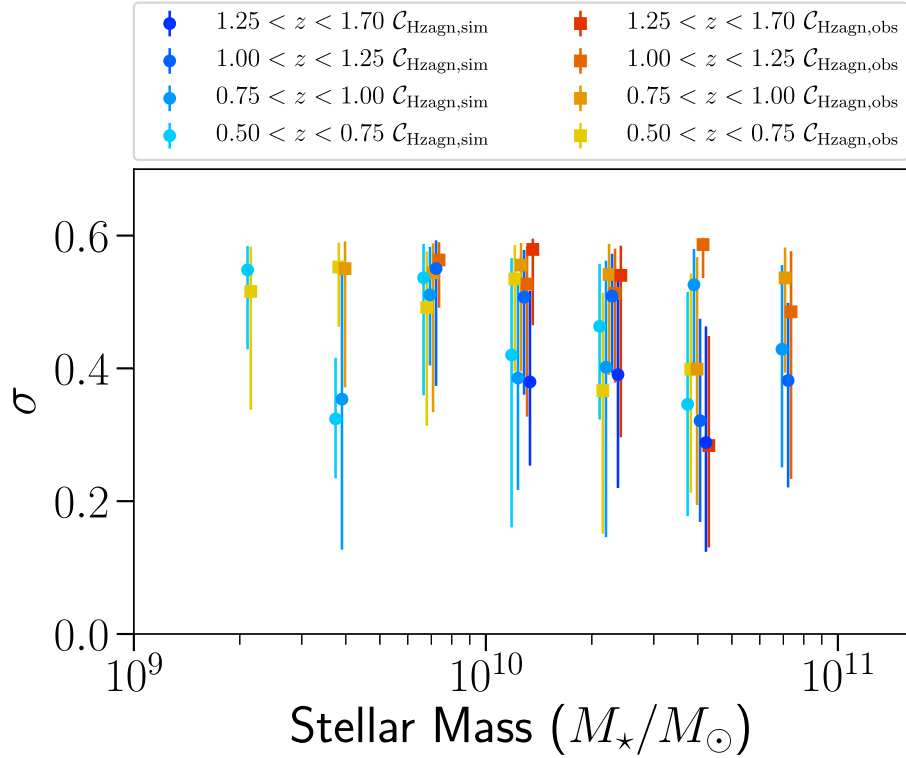
Figure 8. Best-fitting \sigma values for the Horizon-AGN clustering measurements, as a function of galaxy sample threshold stellar mass, for both \mathcal{C}_{\text{Hzagn,sim}} and \mathcal{C}_{\text{Hzagn,obs}} . Data are plotted with small stellar mass offsets for clarity of plot.
