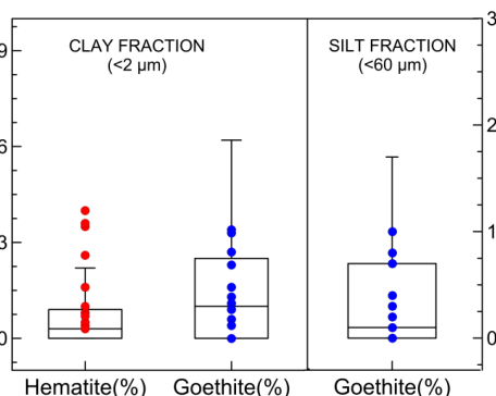
Figure 2. Box and whisker plot showing the full variability of hematite and goethite mass fractions in the clay and silt soil fractions in the dust source regions at the global scale by considering desert source areas as reported in Ginoux et al. (2012) and DB17. Data are from the soil mineralogical database by Journet et al. (2014). Dots indicate hematite and goethite soil content (extracted from Journet et al.) for the nineteen soils used in the CESAM experiments. The Journet database assumes that the iron oxides in the silt fraction consist only of goethite.
