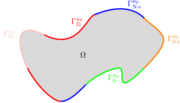
Figure 4: Illustration on an admissible decomposition of \Gamma .
