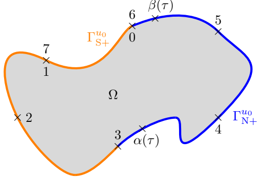
Figure 5: Illustration of the parameterization (2) of \Gamma .
