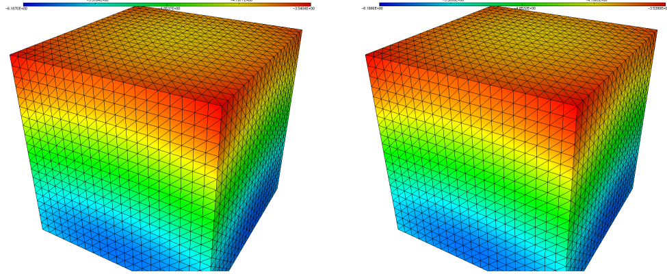
Figure 3: Case t = 0.1 ( d = 3 ): solution u_t (left) and its first-order approximation u_0 + tu'_0 (right).
