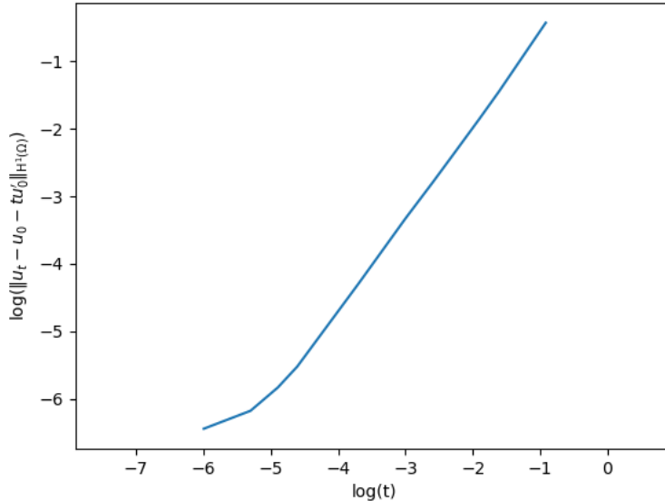
Figure 1: The H^1 -comparison \|u_t - u_0 - tu'_0\|_{H^1(\Omega)} with respect to t in logarithmic scale.
