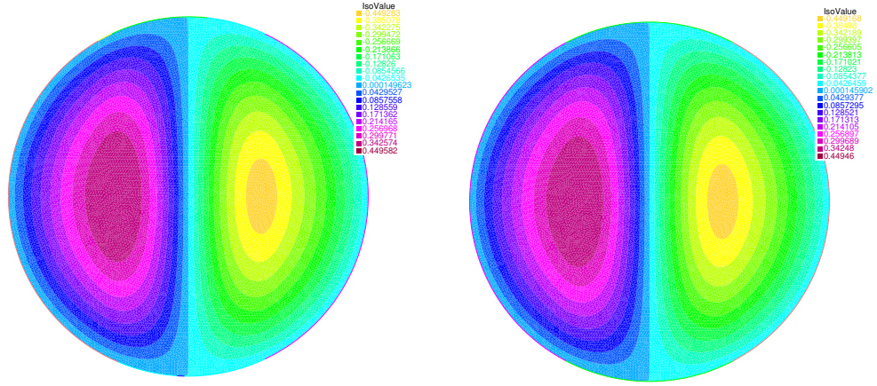
Figure 2: Case t = 0.01 ( d = 2 ): solution u_t (left) and its first-order approximation u_0 + tu'_0 (right).
