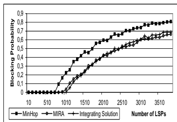
Fig. 6: Blocking probability
