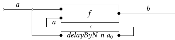
Figure 10. The block diagram of feedForward n a .
