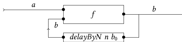
Figure 11. The block diagram of feedBackward n a .
