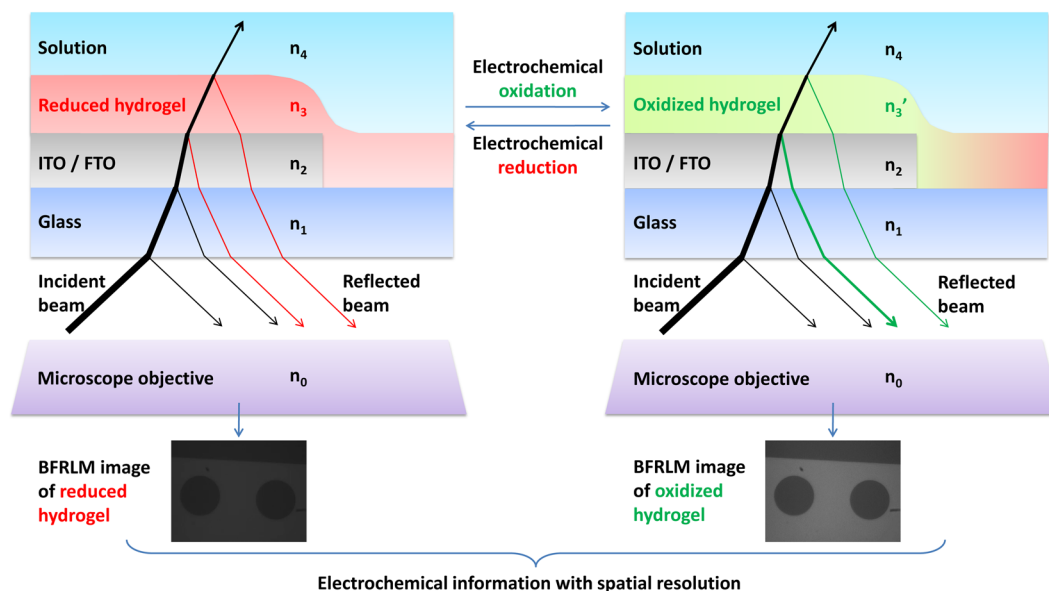
Figure 1. Schematics of BFRLM for increasing the spatial resolution of redox hydrogel-based electrochemical biosensors. The biosensors are obtained by modifying optically transparent metal oxide electrodes fabricated onto planar glass slides with redox hydrogels consisting of cross-linked redox polymers and enzymes. The incident light is refracted and reflected on the different interfaces of the multilayered sensor. The refractive indices of the glass ( n_1 ), of the metal oxide ( n_2 ), of the redox hydrogel ( n_3 ), and of the solution ( n_4 ) define how much of the incident light is returned and analyzed. Only the refractive index of the hydrogels is changing significantly because of the oxidation or reduction of the redox polymer from their composition. Thus, the BFRLM images recorded during our experiments are essentially high-resolution maps of the oxidation state of the redox hydrogels.
