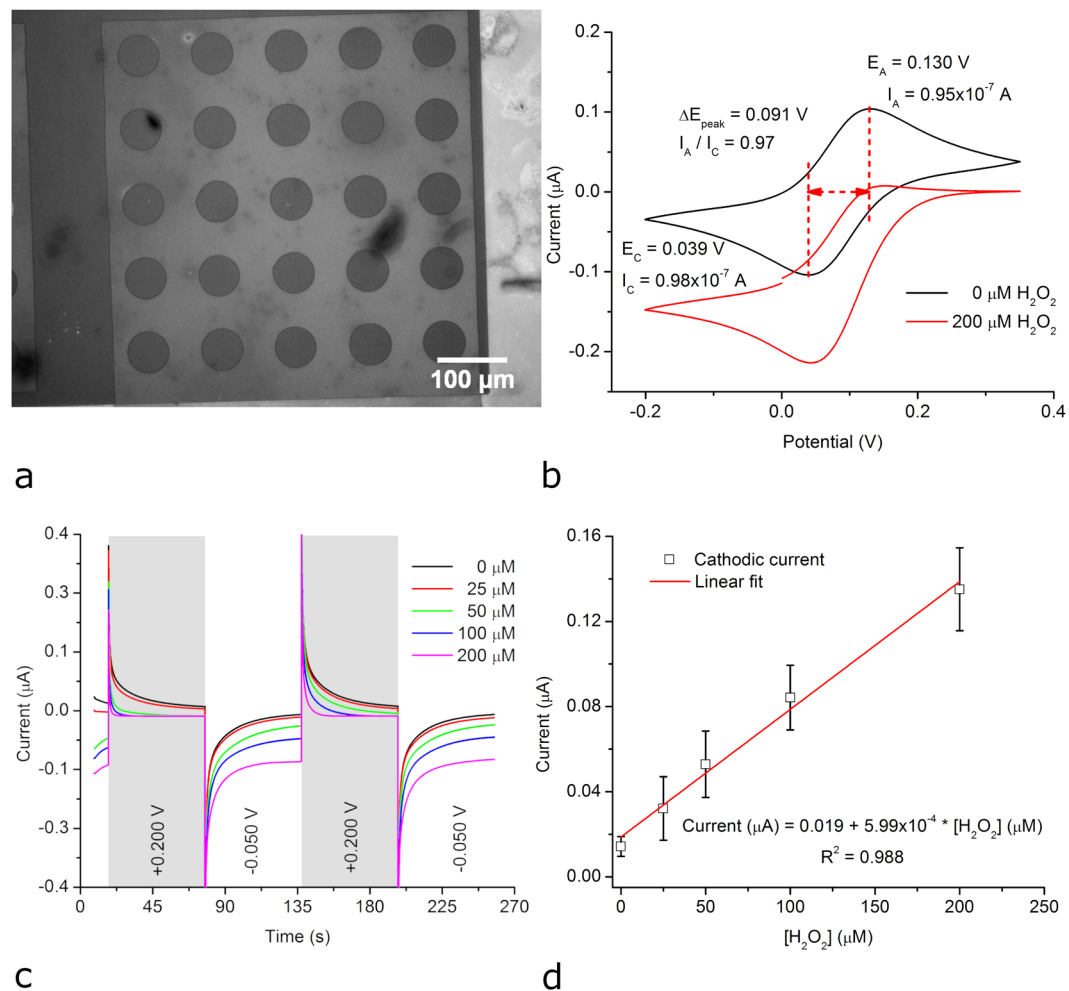
Figure 3. Electrochemical detection of hydrogen peroxide using a FTO electrode modified with HRP-based redox hydrogel. (a) BFRLM image of the FTO electrode. (b) Cyclic voltammograms of the modified FTO electrode recorded at a scan rate of 0.010 \text{ V s}^{-1} in the absence and presence of hydrogen peroxide. (c) Current signal of the modified FTO electrode polarized to potentials oxidizing/reducing the redox polymer while the hydrogen peroxide concentration was stepwise increased. (d) Calibration curve derived from the current values recorded at the end of the second cathodic pulse (at t = 256 \text{ s} ).
