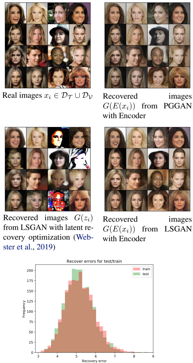
Figure 3. Illustration of latent recovery attack for PGGAN and LSGAN. Real images x_i from the test and train dataset are analyzed with the encoder E then synthesized with the generator G (right). The encoder E , trained on generated images, improves latent recovery in comparison with explicit optimization (Webster et al., 2019). The discrepancy between recovery error (see Eq. 1 is used to perform membership inference attack, which is here unsuccessfully (52% as reported in Table 2).
