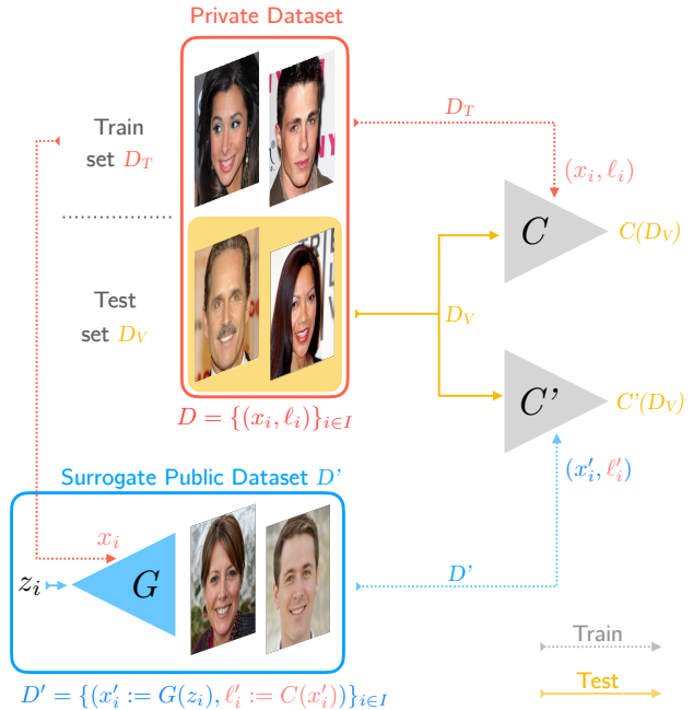
Figure 1. Overview of the proposed framework for creating private data surrogates and its application to train a private task-driven network. In a nutshell, the data surrogate D' is simply obtained by combining image samples from a generator network G (e.g. using GAN) and associating them with plausible labels obtained from a classifier C trained on the private train dataset D_T . From this public dataset, it is possible to train a privacy preserving classifier C' displaying similar performance and accuracy (in practice by comparing C'(D_V) and C(D_V) on a separate validation set D_V ). We further demonstrate empirically that the obtained public dataset D' (and by composition the network C' ) is robust to membership attack that is described in Algorithm 1.
