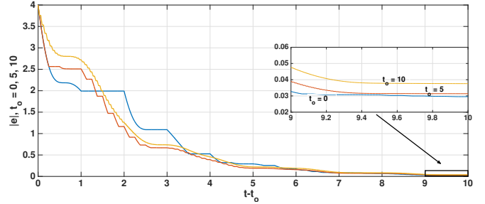
Fig. 5. Convergence rate comparison for different values of t_o under the the weight sequence (5)
