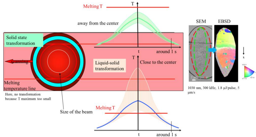
Figure 16. Time evolution of the temperature for a fixed point according to the distance from the focus center in scanning mode at high pulse energy (regime 3 for LNS glass). The right side is the SEM and EBSD images of the cross section of the laser track obtained in the corresponding regime. The color in the EBSD maps is based on \text{LiNbO}_3 space group, coding along the laser polarization direction. Blue dashed line in the SEM image is the beam boundary and red dashed line is the crystallized volume boundary.
