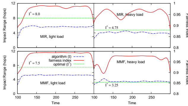
Fig. 7. Impact range and fairness index.
