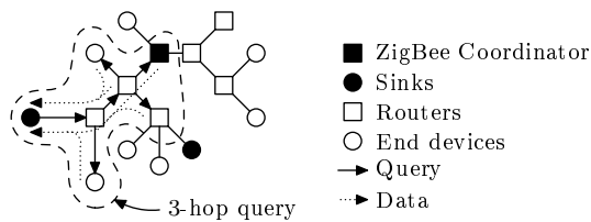
Fig. 2. Multi-sink WSN based on ZigBee tree structure.
