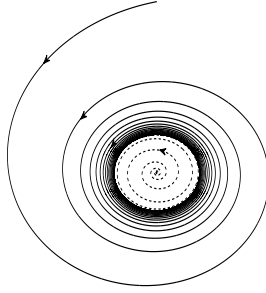
Figure 1. Trajectories of the Stuart-Landau oscillator on the complex plane in the case that \nu_R, \mu_R > 0 . The origin is unstable but all trajectories tend to a stable limit cycle with radius r = \sqrt{\frac{\mu_R}{\nu_R}}
