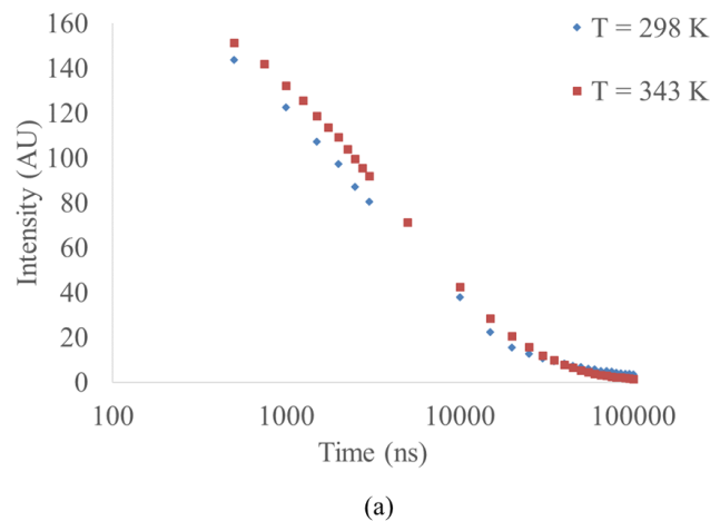
Figure 3: (a) Lifetime curve (on logarithmic scale) for acetone vapour at initial conditions of P = 10,000 Pa and T = 298 K. The same acetone vapour was heated to 343 K.
