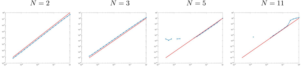
Figure 10: In blue, the plot of \log \varepsilon \mapsto \log(\lambda_N(\varepsilon, \theta) - \lambda_N) , \theta = \frac{7\pi}{20} ; in red, for N = 2, 3 the plot of \log \varepsilon \mapsto \log \varepsilon^2 and for N = 5, 11 the plot of \log \varepsilon \mapsto \log \varepsilon^4 .
