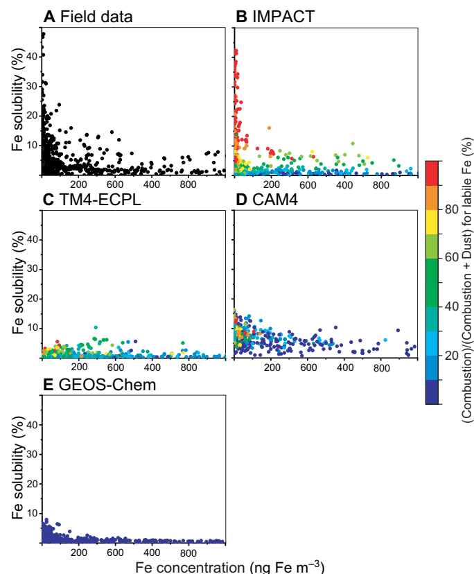
Fig. 1. Atmospheric concentration of total aerosol Fe ( \text{ng m}^{-3} ) versus Fe solubility (%) for simulated estimates (colored circles) and field data (black circles). (A to E) The color represents the (combustion)/(combustion + dust) ratio for labile Fe concentration in aerosols.
