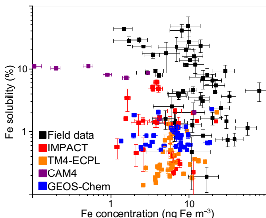
Fig. 5. Fe solubility versus Fe concentration ( \text{ng Fe m}^{-3} ) for field data (black squares), IMPACT (red squares), TM4-ECPL (orange squares), CAM4 (purple squares), and GEOS-Chem (blue squares) over the Southern Ocean ( >45^{\circ}\text{S} ). The vertical lines in symbols correspond to \pm 1 SD for Fe solubility in aerosols.
