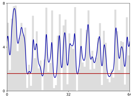
FIG. 12. A random potential (in shaded gray), the corresponding effective potential (the solid blue line), and the fundamental eigenvalue (the horizontal red line).
