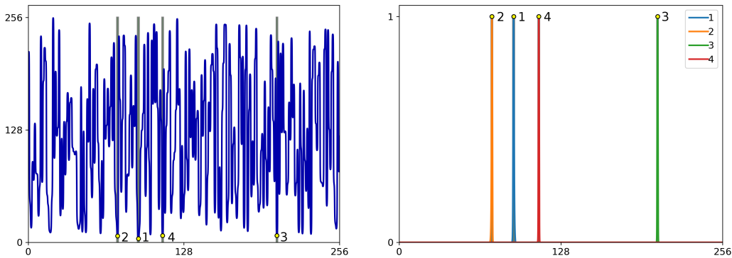
FIG. 6. The effective potential for the potential equal to 64 times that shown on the left of Figure 3, with the four deepest local minima and their wells marked and labeled, and then a comparison with the actual first four eigenfunctions.
