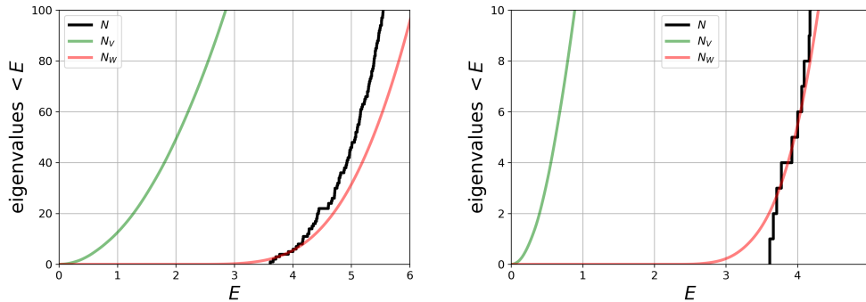
FIG. 19. The eigenvalue counting function N , the Weyl's law approximation N_V , and the effective Weyl's law approximation N_W for the 2D potential of Figure 1, showing the first 100 eigenvalues on left and restricting to the first 10 on right.
