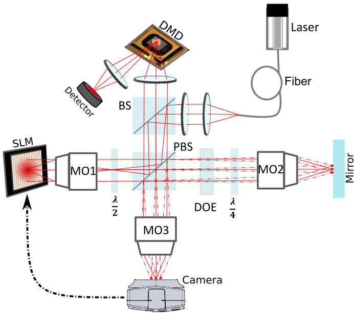
Fig. 1: Scheme of a diffractively coupled photonic network. Network nodes are pixels of a spatial light modulator (SLM), and filtering by a polarizing beam splitter (PBS) brings forward their nonlinearity. A diffractive optical element (DOE) located in the beam-path creates coupling between individual photonic nodes. Network training is implemented with a digital micro-mirror device (DMD) realizing Boolean selection of SLM-pixels transmitted on the output power meter. This system was used to demonstrate learning in the context of a recurrent neural network [17].
