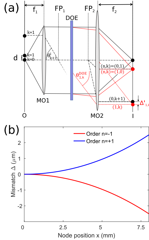
Fig. 2: Scheme to explain the fundamental principle of diffractive coupling. (a) Emitters in the plane O are imaged through microscope objectives MO1, MO2 with respective focal lengths f_1 and f_2 in the plane I. The angle of the principle ray of a node with respect to the optical axis is (\theta_i) and the angle of the +1 diffractive order corresponding to the node is (\theta_{DOE}) . The distance between zero and +1 orders is p and the distance between two nodes is d . (b) Mismatch between the positions of nodes and the coupling term due to diffraction versus node positions in plane O.
