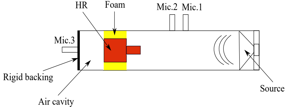
Figure 2: Impedance tube test bench based on the 3 microphones, 2 cavities method used to determine the acoustic performances of the studied devices.
