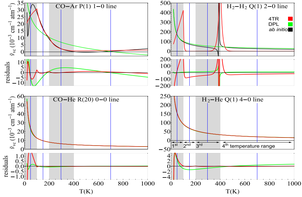
Fig. A1. Temperature dependences of the HT profile frequency of the velocity-changing collisions, \tilde{\nu}_{vc} , [16,33,34] determined from the ab initio \tilde{\nu}_{opt} , \gamma_0 and \delta_0 parameters, see Eqs. 14 and 15, (black lines) and its 4TR and DPL approximations (red and green lines, respectively). To resolve overlapped curves below every graph we show the absolute residuals (the same color notation). The residuals are in the same units as the main plots, i.e., 10^{-3} \text{ cm}^{-1} \text{ atm}^{-1} .
