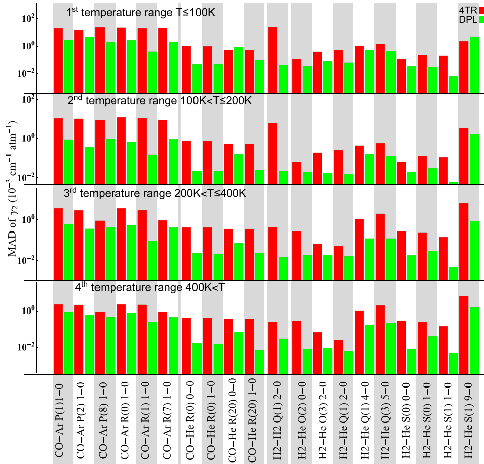
Fig. 7. The MAD for the 4TR and DPL representations of the temperature dependence of the speed dependence of the broadening parameter, \gamma_2 (see text for more details).
