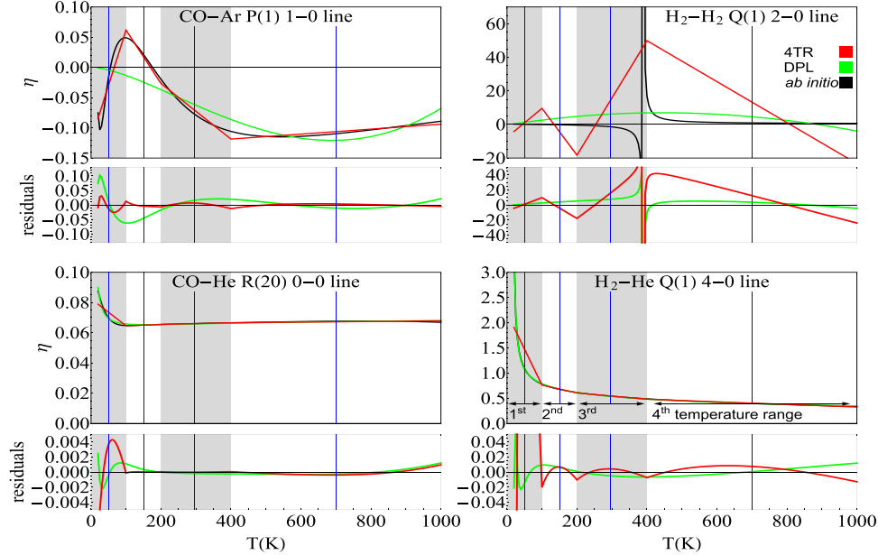
Fig. A2. Temperature dependences of the HT profile correlation parameter, \eta , [16,33,34] determined from the ab initio \tilde{\nu}_{opt} and \delta_0 parameters, see Eq. 15, (black lines) and its 4TR and DPL approximations (red and green lines, respectively). To resolve overlapped curves below every graph we show the absolute residuals (the same color notation). The residuals are in the same units as the main plots, i.e., 10^{-3} \text{ cm}^{-1} \text{ atm}^{-1} .
