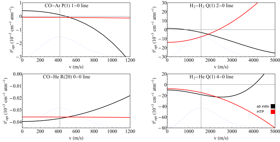
Fig. B2. Ab initio speed dependence of the imaginary part of the Dicke parameter, \tilde{\nu}_{\text{opt}}^i , see Eq. C.6b, (black lines) and its approximation adopted in the HT profile, see Eq. (B.2) (red lines). The Maxwell-Boltzmann distributions of the molecular velocities are shown as blue lines and the thin black vertical lines mark the most probable speed. All the data presented here are for T = 296 K.
