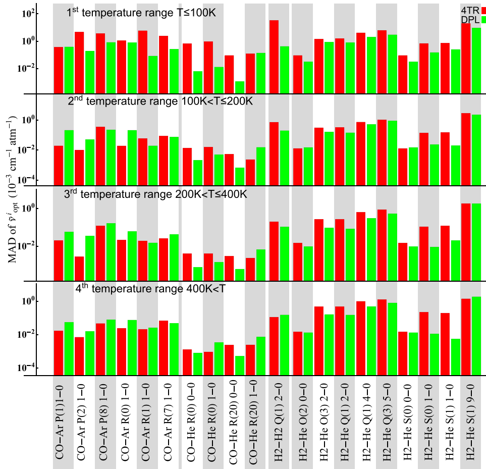
Fig. 12. The MAD for the 4TR and DPL representations of the temperature dependence of the imaginary part of the Dicke parameter, \tilde{\nu}_{\text{opt}}^i (see text for more details).
