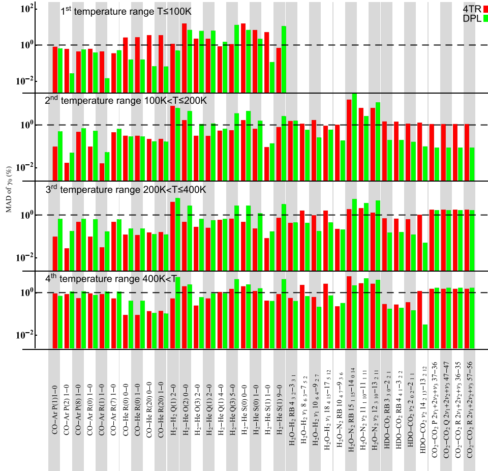
Fig. 3. The relative MAD for the 4TR and DPL representations of the temperature dependence of the pressure broadening parameter \gamma_0 (see text for more details). The 1% level is indicated with the horizontal black dashed lines. The first temperature range is not covered by the semiclassical MCRB calculations.
