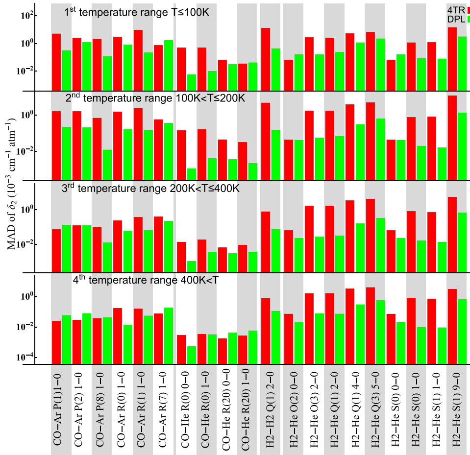
Fig. 8. The MAD for the 4TR and DPL representations of the temperature dependence of the speed dependence of the shift parameter, \delta_2 (see text for more details).
