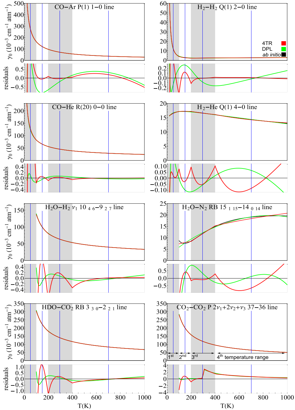
Fig. 1. Ab initio temperature dependences of the pressure broadening parameter \gamma_0 , (black lines) and its 4TR and DPL approximations (red and green lines, respectively). To resolve overlapped curves below every graph we show the absolute residuals (the same color notation). The first temperature range is not covered by the semiclassical MCRB calculations. The residuals are in the same units as the main plots, i.e., 10^{-3}\text{cm}^{-1}\text{atm}^{-1} .
