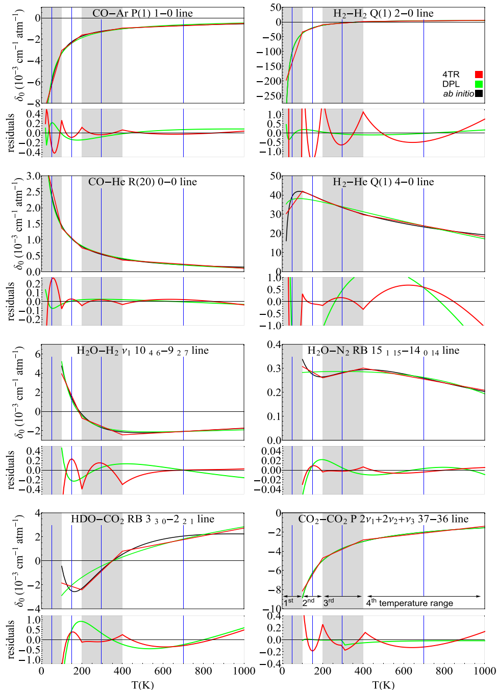
Fig. 2. Ab initio temperature dependences of the pressure shift parameter \delta_0 , (black lines) and its 4TR and DPL approximations (red and green lines, respectively). To resolve overlapped curves below every graph we show the absolute residuals (the same color notation). The residuals are in the same units as the main plots, i.e., 10^{-3} \text{ cm}^{-1} \text{ atm}^{-1} . The first temperature range is not covered by the semiclassical MCRB calculations.
