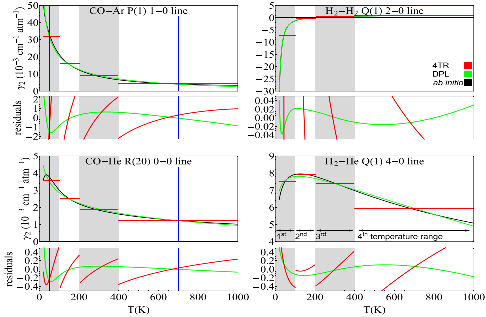
Fig. 5. Temperature dependence of the speed dependence of the broadening parameter, \gamma_2 . The black lines are the functions determined from our ab initio calculations, while red and green ones are the 4TR and DPL representations, respectively. To resolve overlapped curves below every graph we show the absolute residuals (the same color notation). The residuals are in the same units as the main plots, i.e., 10^{-3} \text{cm}^{-1} \text{atm}^{-1} .
