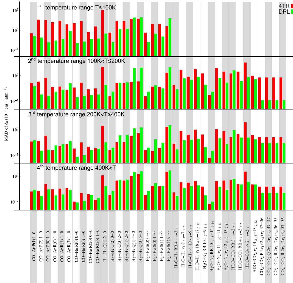
Fig. 4. The MAD for the 4TR and DPL representations of the temperature dependence of the pressure shift parameter, \delta_0 (see text for more details). The first temperature range is not covered by the semiclassical MCRB calculations.
