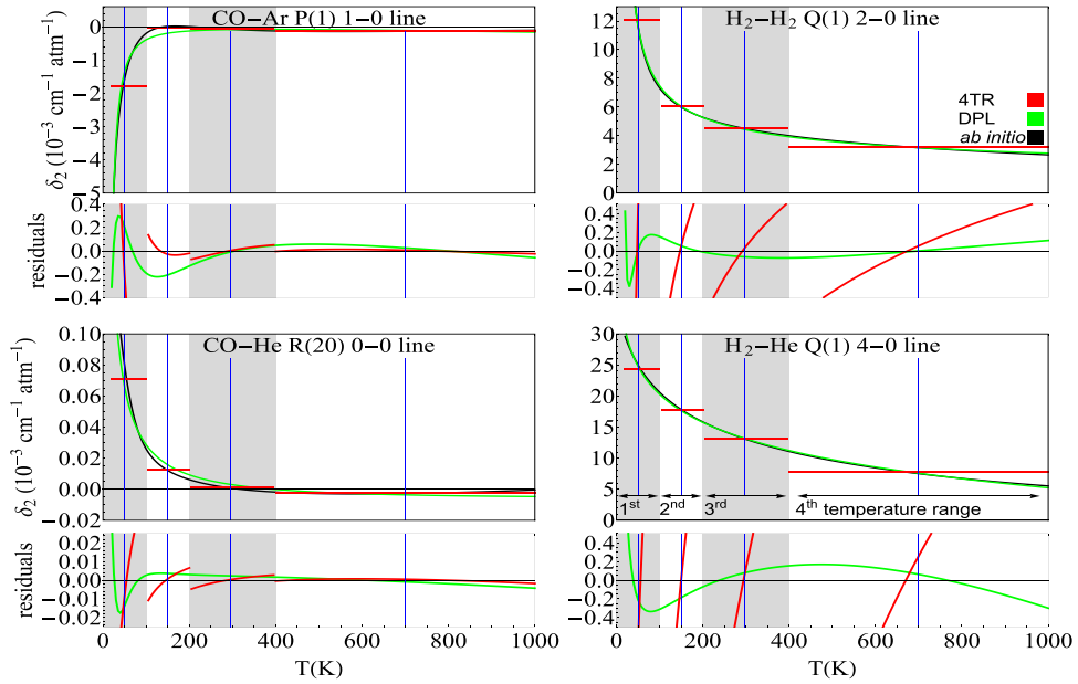
Fig. 6. Temperature dependence of the speed dependence of the shift parameter, \delta_2 . The black lines are the functions determined from our ab initio calculations, while red and green ones are the 4TR and DPL representations, respectively. To resolve overlapped curves below every graph we show the absolute residuals (the same color notation). The residuals are in the same units as the main plots, i.e., 10^{-3} \text{ cm}^{-1} \text{ atm}^{-1} .
