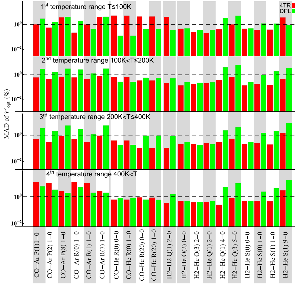
Fig. 11. The MAD for the 4TR and DPL representations of the temperature dependence of the real part of the Dicke parameter, \tilde{\nu}_{opt}^r (see text for more details).
