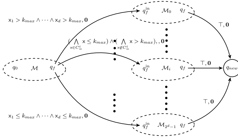
Fig. 4. Machine \mathcal{M}' with 2^d copies of \mathcal{M}
