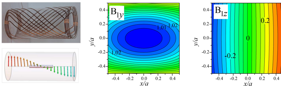
Figure 1: Left: photograph of a spiral coil used for z-encoding in low-field TRASE experiments 3 and sketch of the transverse rf field directions it generates. The spiral coil pitch is k=0.12\text{ cm}^{-1} . Right: computed maps of the transverse and longitudinal field components in the central xy plane, scaled to the field B_C at the coil centre (coil radius: a=6.5\text{ cm} ). Over the same domain, B_{1x}/B_C (not displayed) remains smaller than 0.02, hence the transverse field has a very uniform direction and amplitude. As expected for this near-uniform field, B_{1z} only depends on x , with the expected linear variation (see text) over a wide domain.
