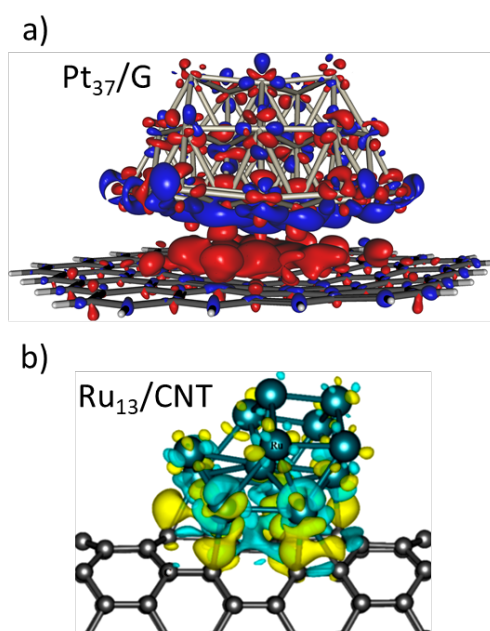
Figure 26. Contour plots of differential charge density of: a) \text{Pt}_{37}/\text{G} ; in blue (red), increase (decrease) of the electron density upon interaction; reprinted with permission from ref 498 Copyright 2019 from AIP Publishing; and b) \text{Ru}_{13}/\text{CNT} . The charge accumulation region is rendered in yellow, while the charge depletion region is in blue. Reprinted with permission from Zhou, S.; et al. J. Phys. Chem. C 2018 , 122 , 9091-9100. 509 . Copyright 2018 from the American Chemical Society.
