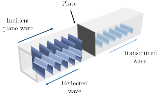
Figure 1: 3-D scheme of the problem in transmission. Dark blue represents the incident plane wave generated by the source, medium blue represents the sound wave that is reflected by the plate and soft blue represents the transmitted wave. The plate is represented in grey.
