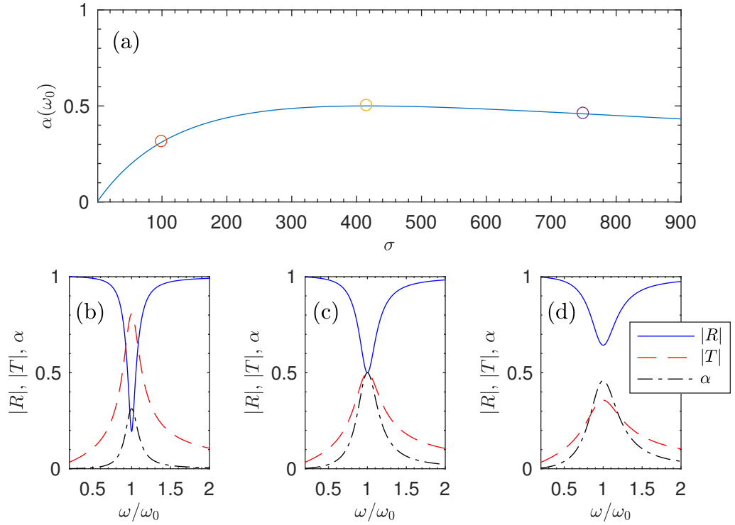
Figure 6: Analysis of the scattering parameters on the losses of the system. (a) represents the absorption of the system at the resonance frequency of the system as the losses increases. Dots in (a) represents the analyzed cases in (b), (c) and (d). (b), (c) and (d) show the scattering coefficients for three particular values of the losses: \sigma = 100 \text{ s}^{-1} , \sigma = 416 \text{ s}^{-1} , \sigma = 750 \text{ s}^{-1} respectively.
