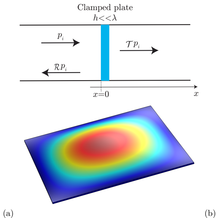
Figure 2: (a) 1-D scheme of the problem in transmission. (b) First mode (piston mode) of the plate.
