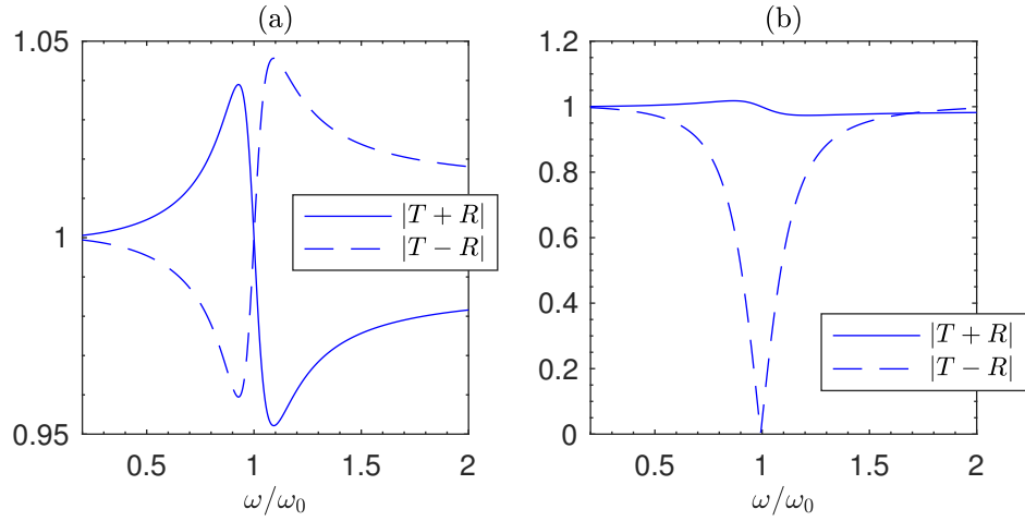
Figure 5: Analysis of the eigenvalues of the system. (a) represents the case without losses ( \sigma = 0 ) and (b) represents the case with losses ( \sigma = 416 \text{ s}^{-1} ). (a) [(b)] represents the absolute value of the both eigenvalues of the system, |T + R| (blue continuous line) and |T - R| (blue dashed line) for the lossless [lossy] case. In all the cases the dependence is shown with respect to the normalized frequency with respect to the resonant frequency of the plate, \omega_0 .
