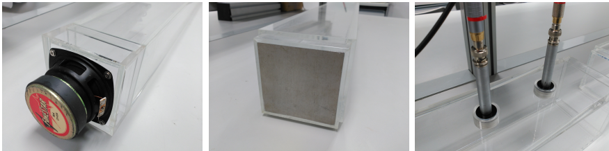
Figure 7: Experimental set up for measurements.
