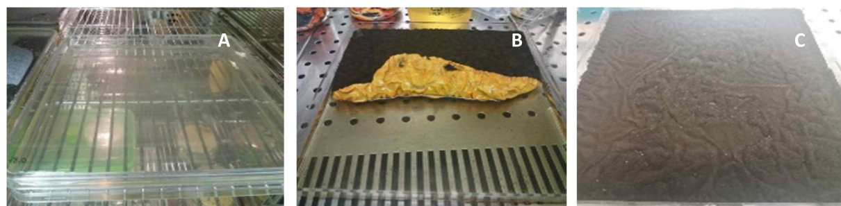
Fig. 7. A. tubingensis morphologies under different oxidative stress in bioassay plate at pH 5 and 28°C during 9 days, static conditions.
