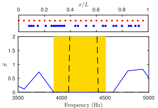
FIG. 3. (Color online) Structure factor for the periodic and stealth material. Upper panel represents both the periodic configuration [red squares (■)] and the stealth configuration [blue dots (●)]. The positions of the scatterers in the stealth configurations are: x_n/L = [0.083, 0.099, 0.116, 0.15, 0.211, 0.256, 0.273, 0.289, 0.305, 0.322, 0.338, 0.354, 0.439, 0.46, 0.523, 0.582, 0.653, 0.673, 0.735, 0.755, 0.8, 0.854, 0.871, 0.904, 0.93] . Lower panel shows the structure factor for the periodic distribution [black dashed line, (---)] and for the stealth material [blue continuous line (—)]. Yellow area shows the frequency range of the optimization.
