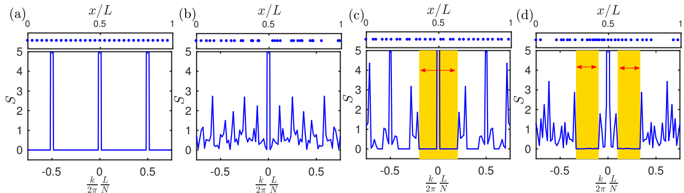
FIG. 2. (Color online) Representation of the structure factor for (a) a periodic, (b) a random, (c) a hyperuniform and (d) a stealth distributions of N = 30 scatterers. The hyperuniform configuration is obtained to reduce scattering in the range |k| \leq |k_B/2.5| (where k_B = \pi N/L is the Bragg condition of the corresponding periodic configuration). The stealth configuration is optimized for k_B/5 \leq |k| \leq k_B/1.5 . The target range of frequencies of the two last cases are shown by the yellow area in (c) and (d).
