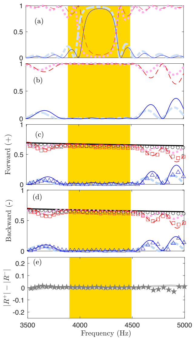
FIG. 5. (Color online) Analysis of the scattering produced by the stealth material. In the Figure the transmission, T^2 , [reflection, R^2 ,] analytically and numerically calculated are represented by the shaded pink (---) and red dashed (---) lines respectively [shaded blue (---) and blue continuous (---) lines respectively] and the experimental values are represented by red squares ( \square ) [blue triangles ( \triangle )]. (a) Scattering coefficients of (a) the periodic distribution in the lossless case, (b) the stealth material in the lossless case, (c) and (d) the stealth material in the lossy case excited from the forward and backward incidence directions respectively. Black (—) continuous line and black circles ( \circ ) represent the transmission coefficient of the empty waveguide, theoretical and experimental values respectively. (e) |R^+| - |R^-| from the TMM (—) and experimental results ( \star ).
