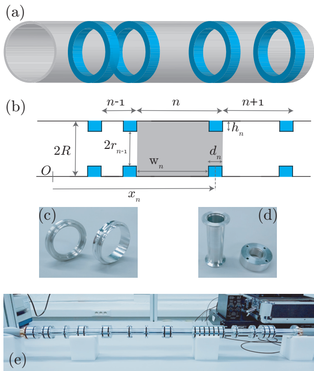
FIG. 4. (Color online) Schematics of both a three dimensional view (a) and the cross section (b) of the cylindrical waveguide along the n -th diaphragm. (c-e) Experimental set-up. (c) Connections: left diaphragme and flat connection for empty tube. (d) Separators. (e) Picture of the stealth material.
