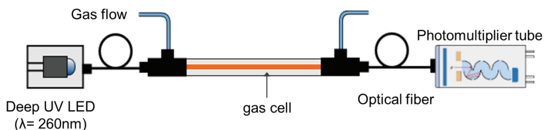
Figure 2. Schematic of experimental setup. Aluminum HCW is employed as a gas cell, coupled with UV LED and PMT via optical fibre.
