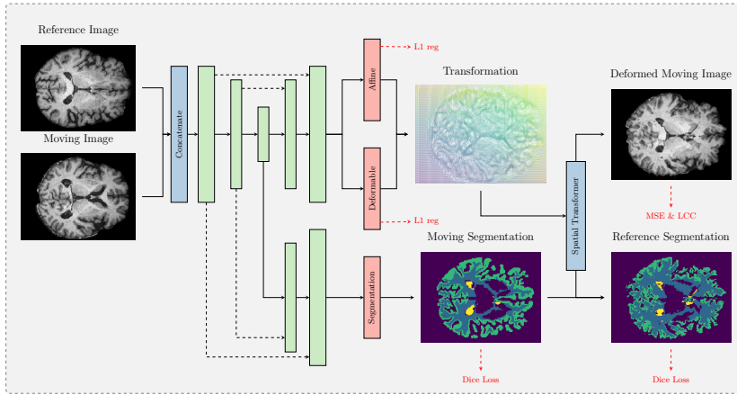
Fig. 1: The employed architecture with the registration and segmentation parts. Green layers: convolutional blocks with successive Convolution, LeakyReLU and down/upsampling operations.
