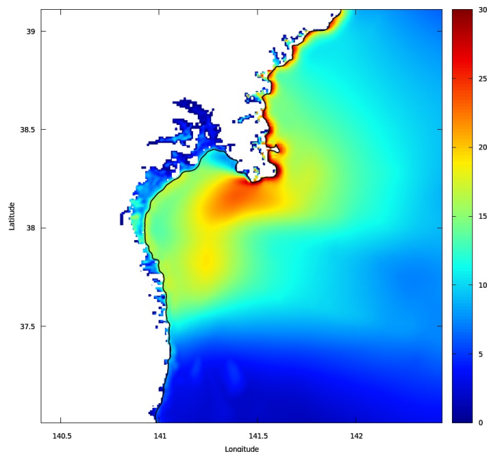
Figure 10. Detail of flooding in the Ofunato, Miyagi and Fukushima districts. The black line indicates the normal coastline. The colorscale is the maximum flood level (maximum water elevation above normal) in meters ( http://basilisk.fr/src/examples/tohoku.c ).
