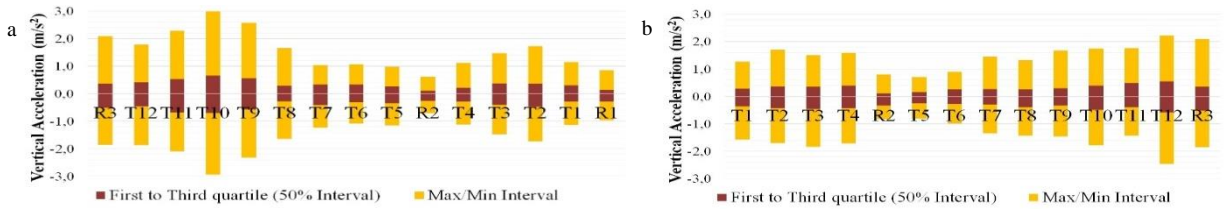
Fig. 6. (a) Vehicle vertical acceleration toward Imola; (b) Vehicle vertical acceleration towards Forlì
