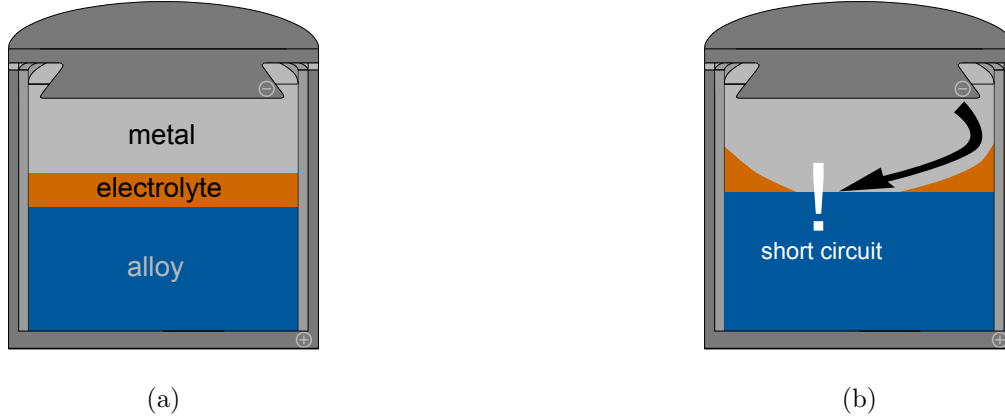
FIG. 1. Sketch of a liquid metal battery (a) and short-circuit due to a deformation of the electrolyte layer (b).
