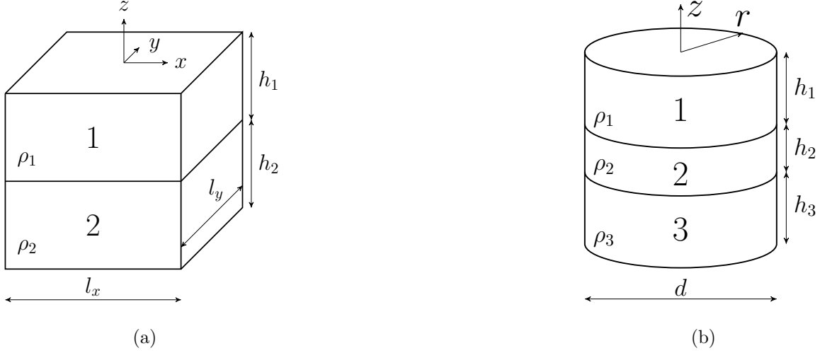
FIG. 4. Sketch of a an aluminium reduction cell (a) and liquid metal battery (b).
