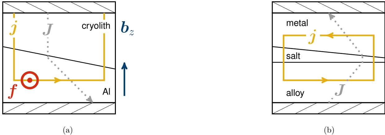
FIG. 2. Cross section of an aluminium reduction cell (a) and a liquid metal battery (b) with tilted interface 40,41 . \mathbf{J} denotes the total cell current, \mathbf{j} the perturbed or compensation current, \mathbf{B}_{0,z} a vertical magnetic field and \mathbf{f} the resulting Lorentz force.
