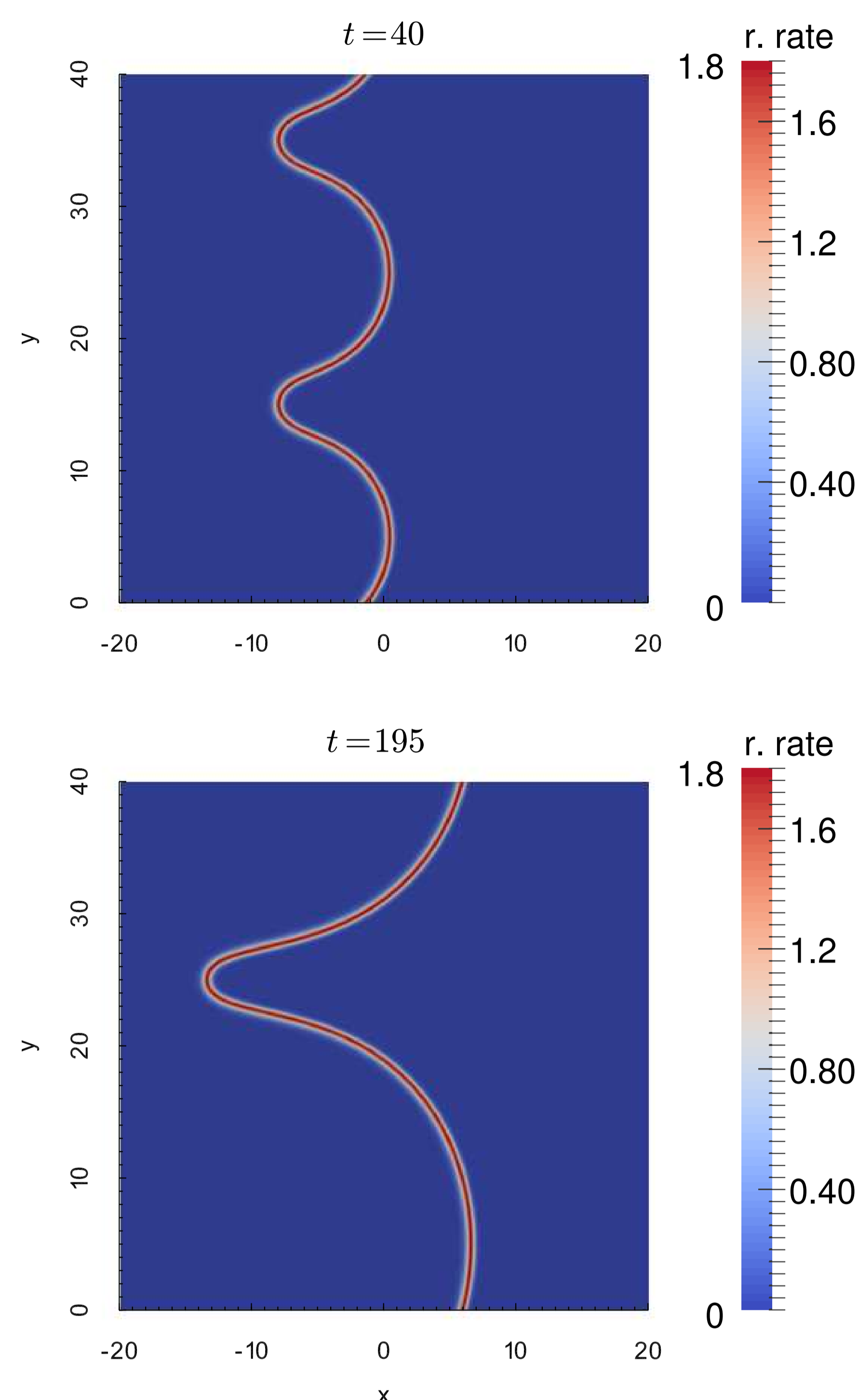
Fig. 1: Reaction rate field for h/\delta_T \rightarrow 0 showing the flame front curvature at different instants. Flame propagates from left to right.
