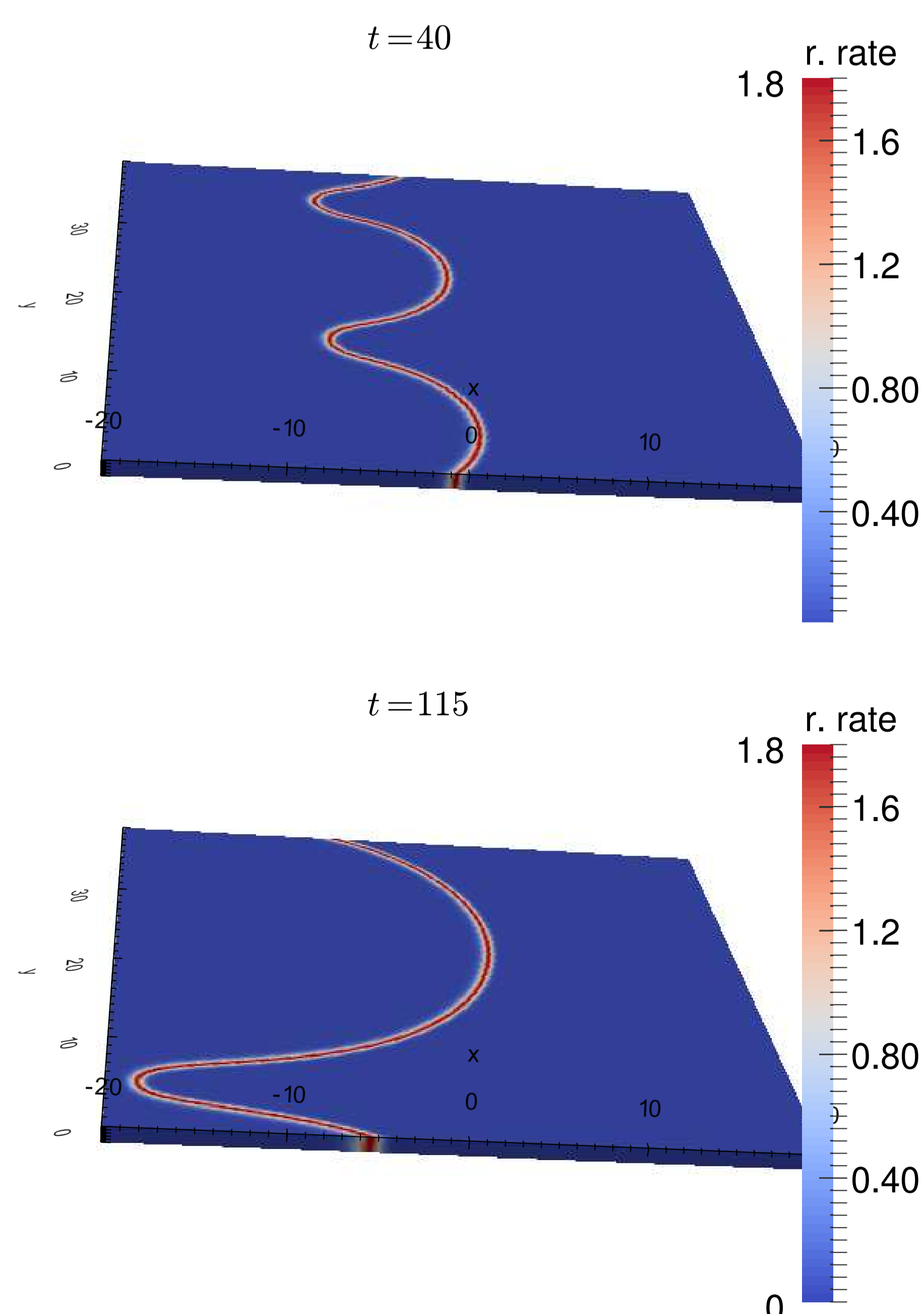
Fig. 2: Reaction rate field for h/\delta_T = 1 showing the flame front curvature at different instants. Flame propagates from left to right.
