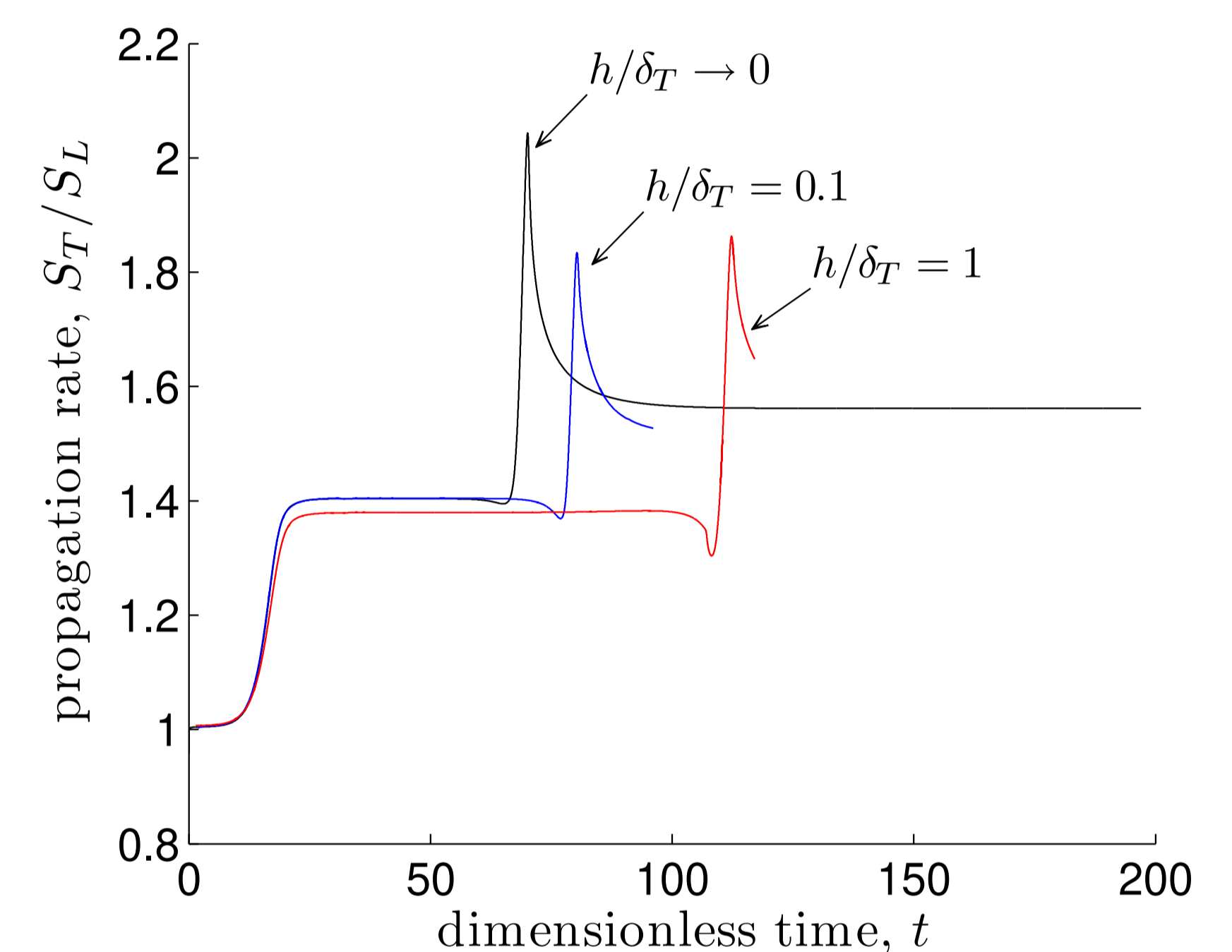
Fig. 3: Propagation rate as function of time for different cell gaps h/\delta_T .
